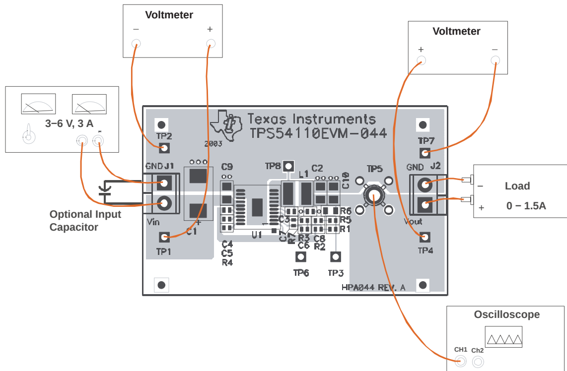
Figure 2-1. Connection Diagram
