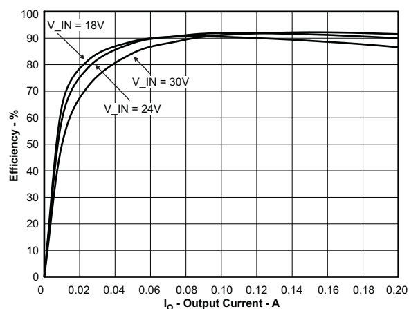
Figure 1. TPS54060EVM-590 Efficiency
