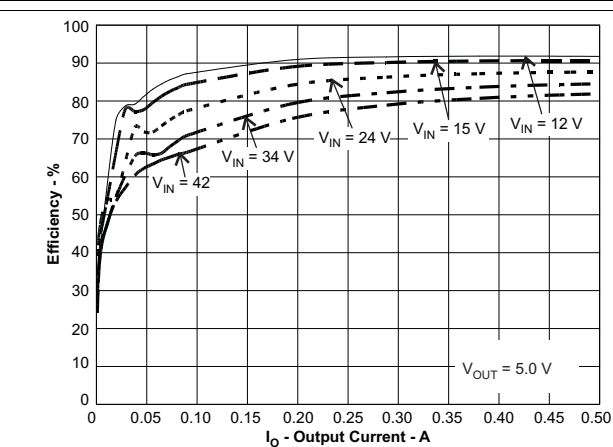
Figure 59. Efficiency vs Load Current
