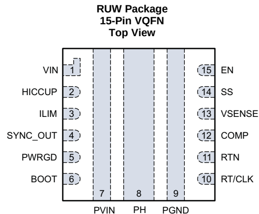
Pin Functions
