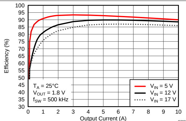
Figure 41. Efficiency
