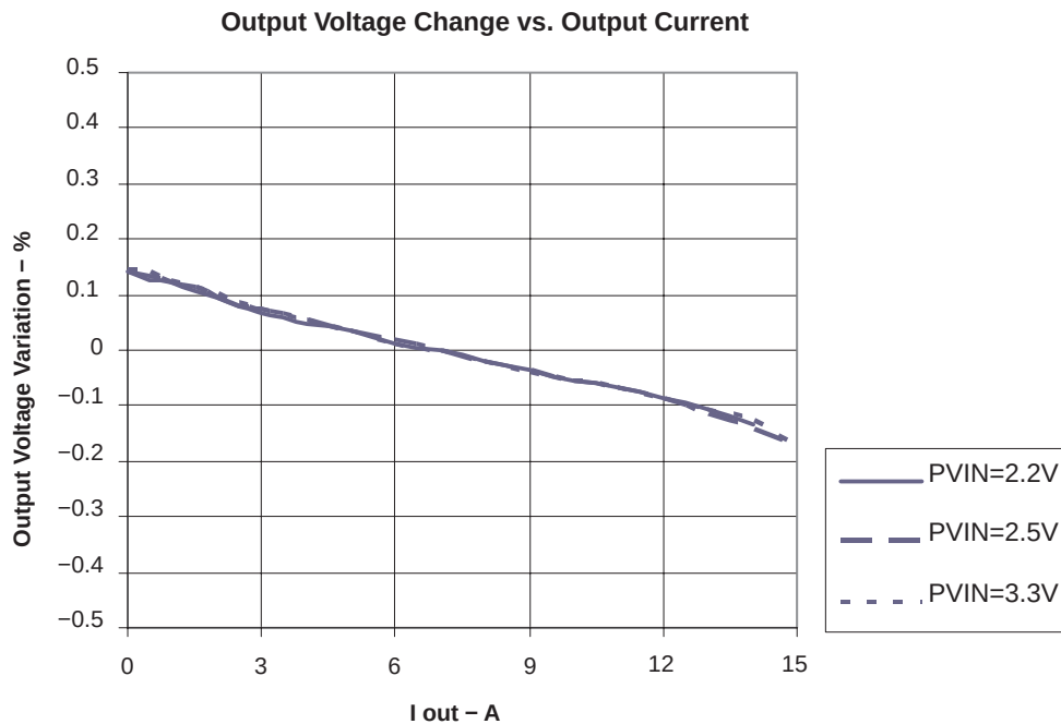
Figure 2-2. Load Regulation
