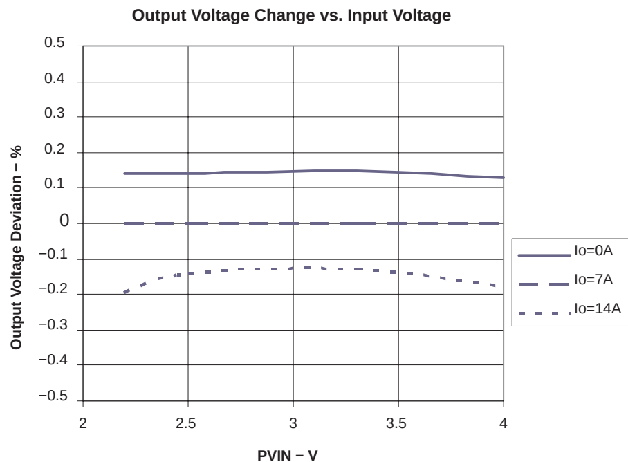
Figure 2-3. Line Regulation
