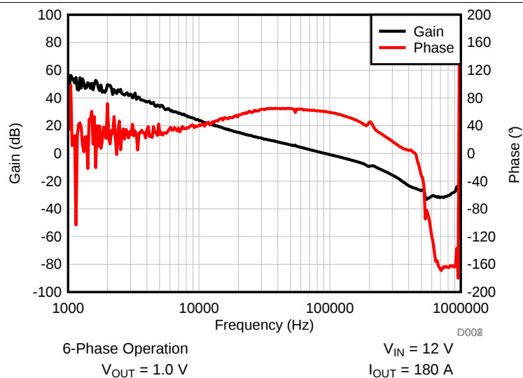
Figure 117. Bode Plot
