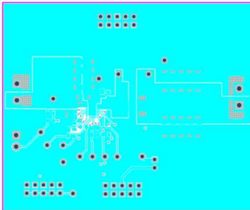
Figure 6. TPS53513EVM-587 Top Copper
