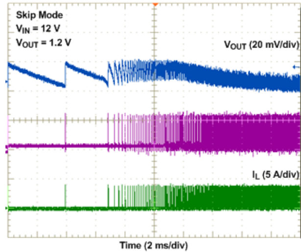
Figure 16. DCM to CCM Transition
