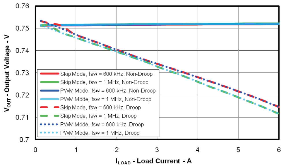
Figure 5. Load Regulation
