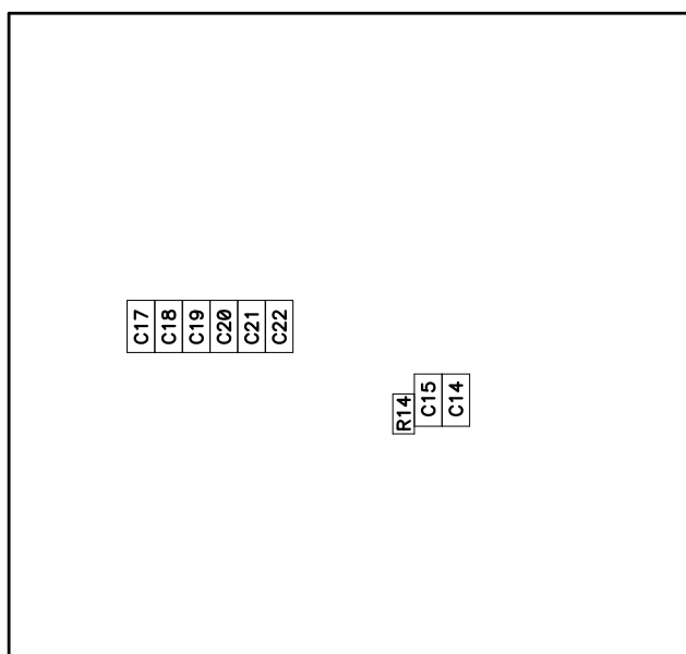
Figure 18. TPS53317EVM-750 Bottom Layer Assembly Drawing (bottom view)
