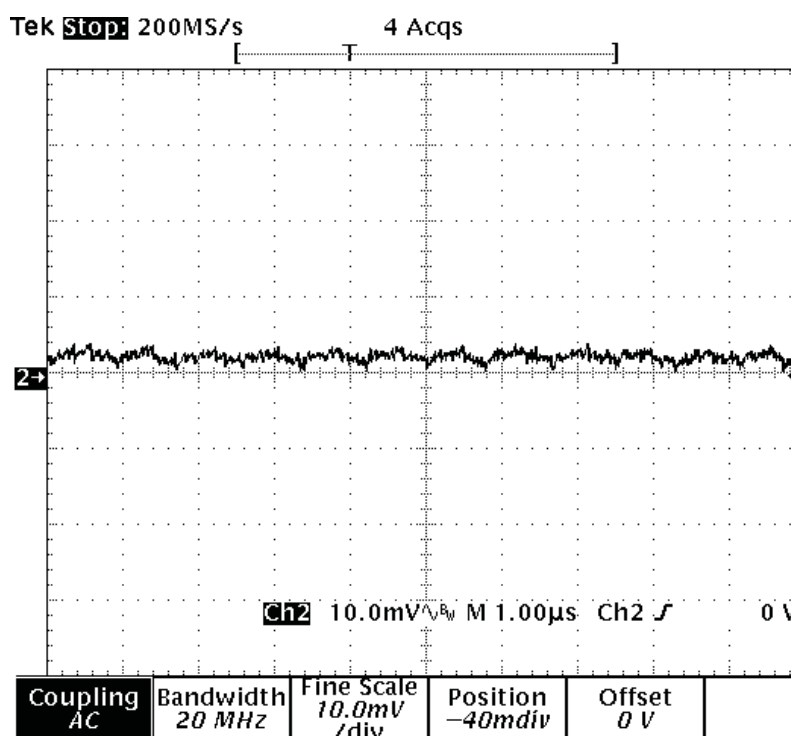
Figure 9. Output Ripple (1.5-V V_{IN} , 0.75-V V_{OUT} , 3-A I_{OUT} , f_{SW} = 1 MHz)
