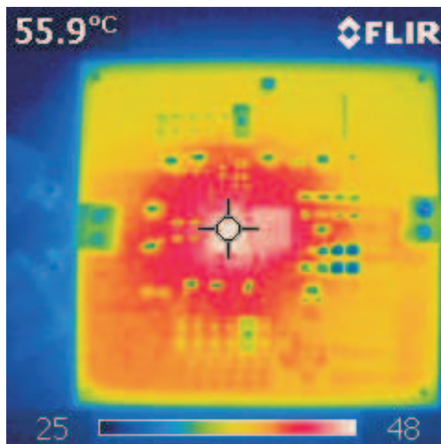
Figure 19. Thermal Image (6-V VIN, 1.5-V VOUT, 5-A IOUT, FCCM Mode, f_{sw} = 2.0 MHz)
