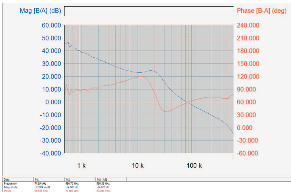
Figure 18. Loop Gain (5-V VIN, 1.5-V VOUT, 5-A IOUT, HEF Mode, f_{sw} = 750 kHz)
