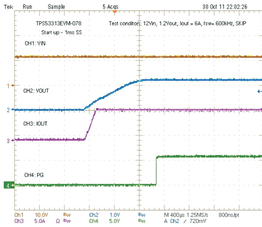
Figure 13. Start-Up Waveform (12-V VIN, 1.2-V VOUT, 6-A IOU, 1-ms SS)
