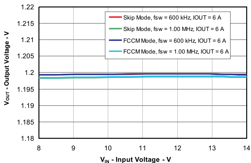
Figure 6. Line Regulation
