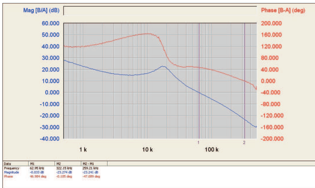
Figure 18. Loop Gain (12-V VIN, 1.2-V VOUT, 6-A IOUT, Skip Mode, f_{sw} = 600 kHz)
