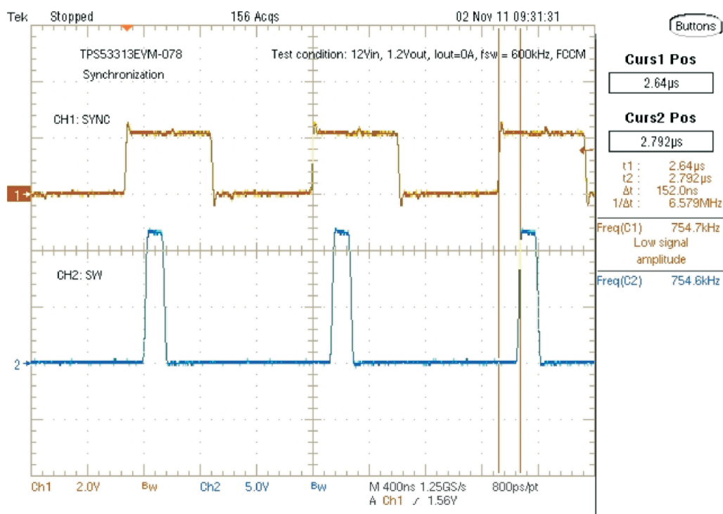
Figure 17. Synchronization Waveform (12-V VIN, 1.2-V VOUT, 0-A IOUT, free-running frequency = 600 kHz, SYNC frequency = 750 kHz)
