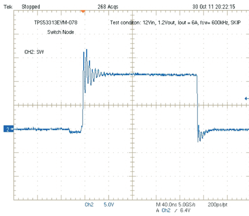
Figure 12. Switching Node at Full Load (12-V VIN, 1.2-V VOUT, 6-A, Skip Mode, f_{sw} = 600 kHz)
