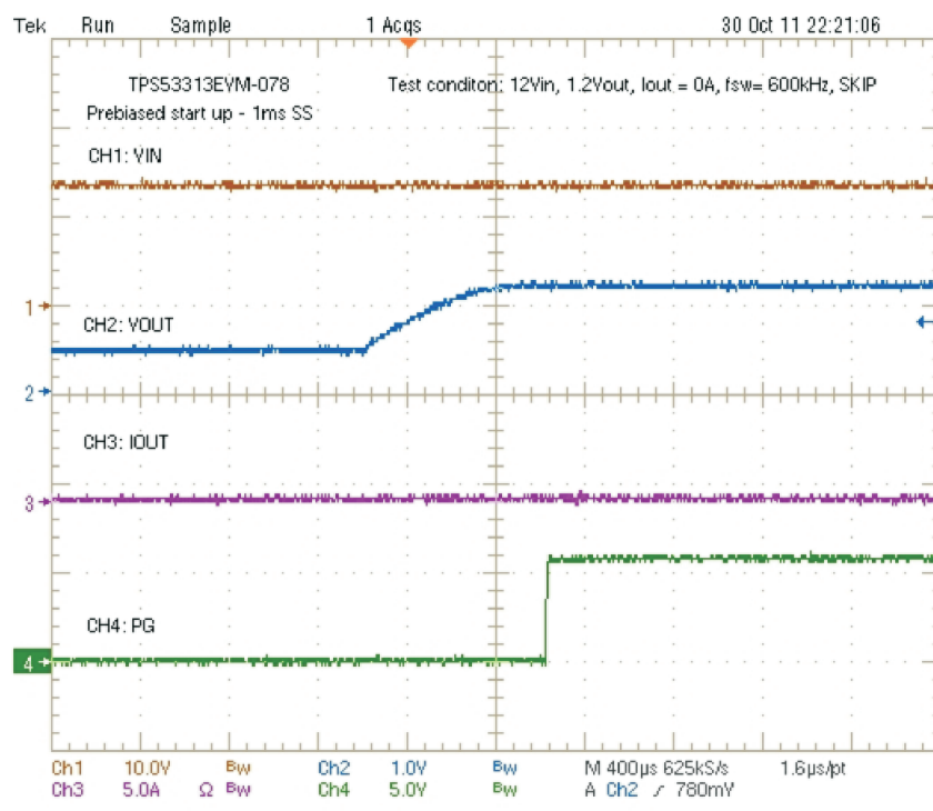
Figure 14. Pre-bias Start-Up Waveform (12-V VIN, 1.2-V VOUT, 0-A IOU, 1-ms SS)
