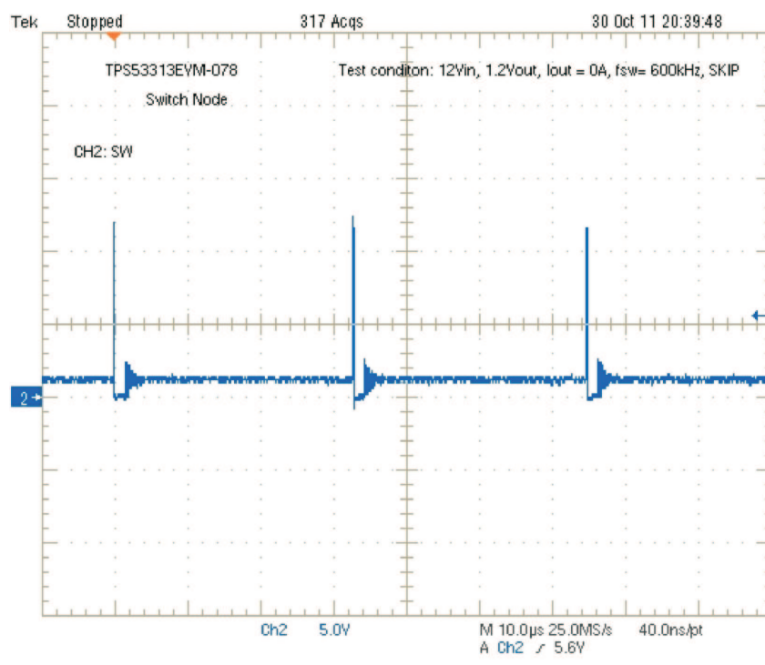
Figure 11. Switching Node at No Load (12-V VIN, 1.0-V VOUT, 0-A, Skip Mode, f_{sw} = 600 kHz)
