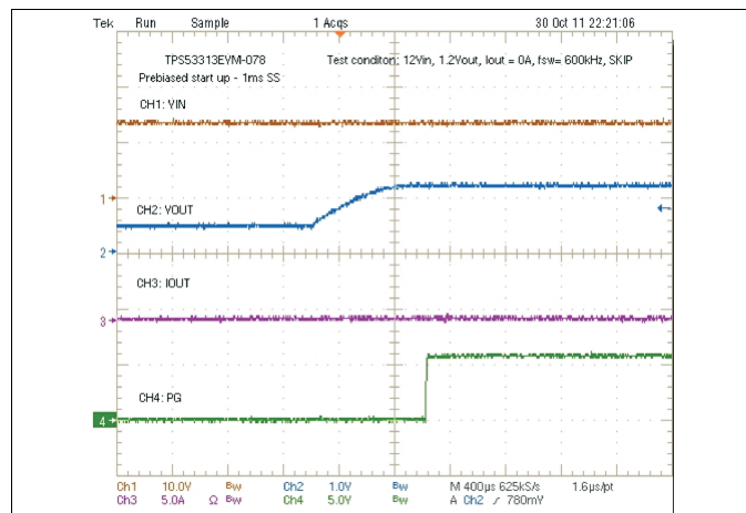
Figure 23. Pre-bias Start-Up Waveform
