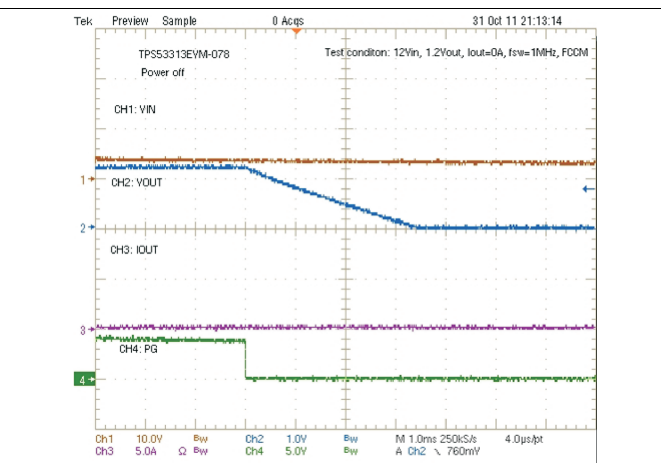
Figure 24. Shut-Down Waveform
