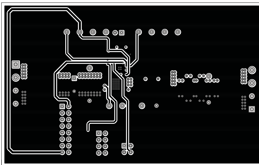
Figure 20. TPS53219EVM-690 Layer-3 Copper, Top View
