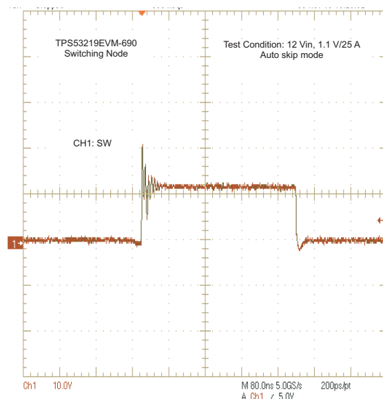
Figure 9. Switching Node
