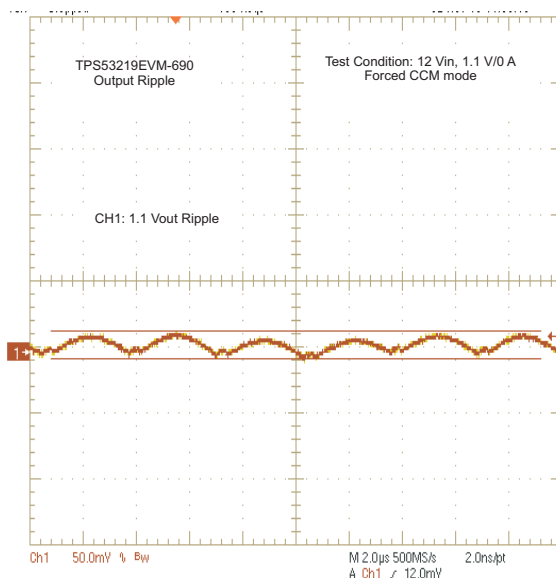
Figure 8. Output Ripple
