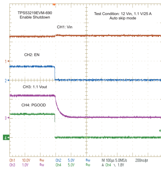
Figure 11. Enable Turnoff
