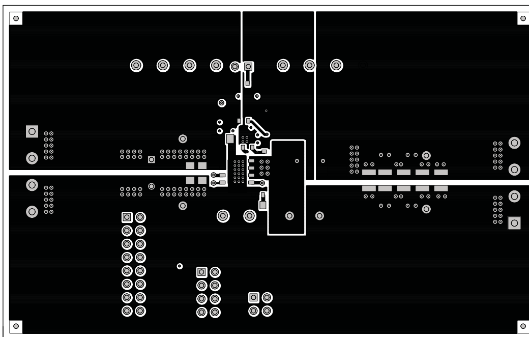
Figure 18. TPS53219EVM-690 Top Copper, Top View
