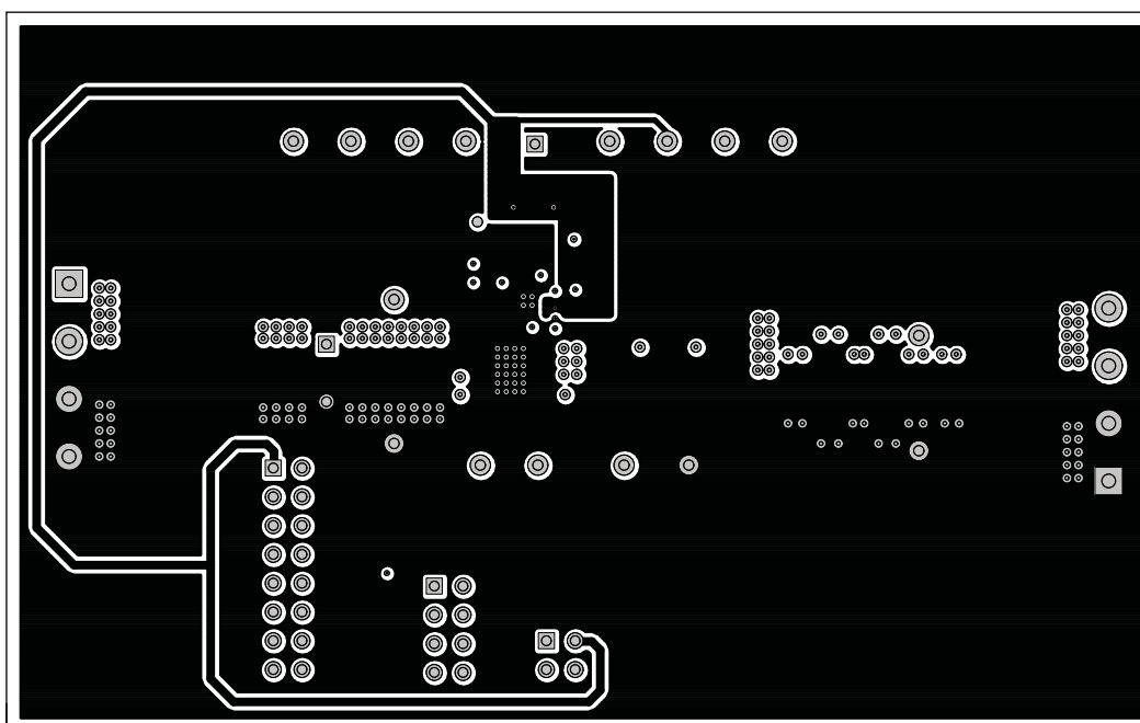
Figure 19. TPS53219EVM-690 Layer-2 Copper, Top View
