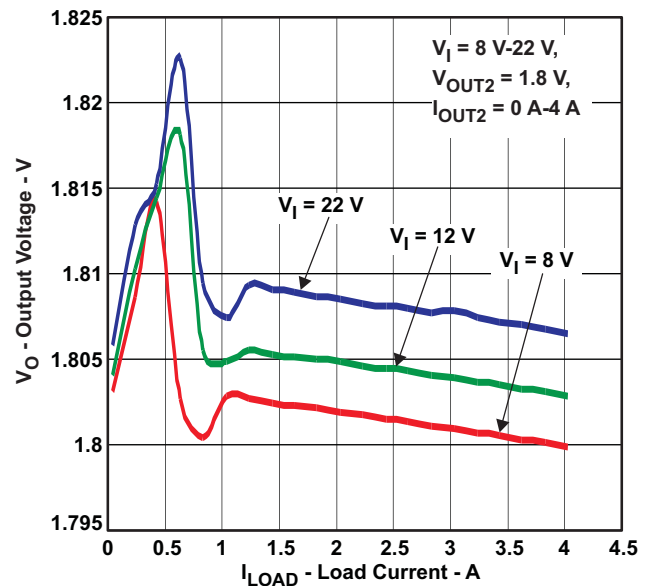
Figure 7. Output Voltage vs Load
