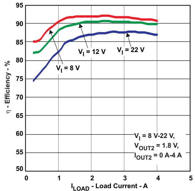
Figure 5. Efficiency vs Load
