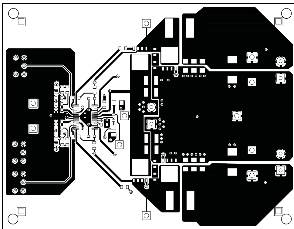
Figure 14. Top Layer
