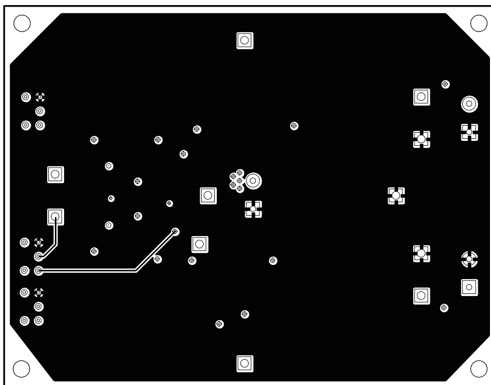
Figure 16. Internal Layer 1
