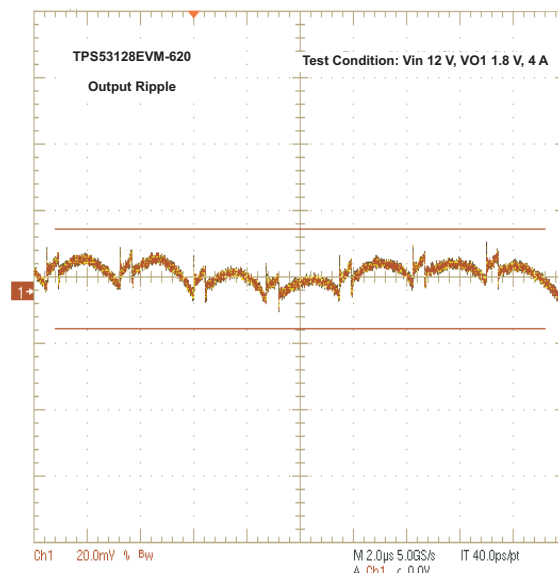
Figure 9. Output Voltage Ripple
