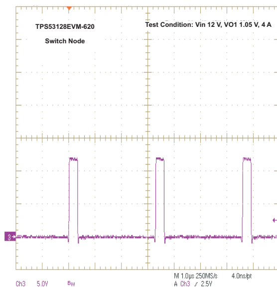
Figure 10. Switching Waveform
