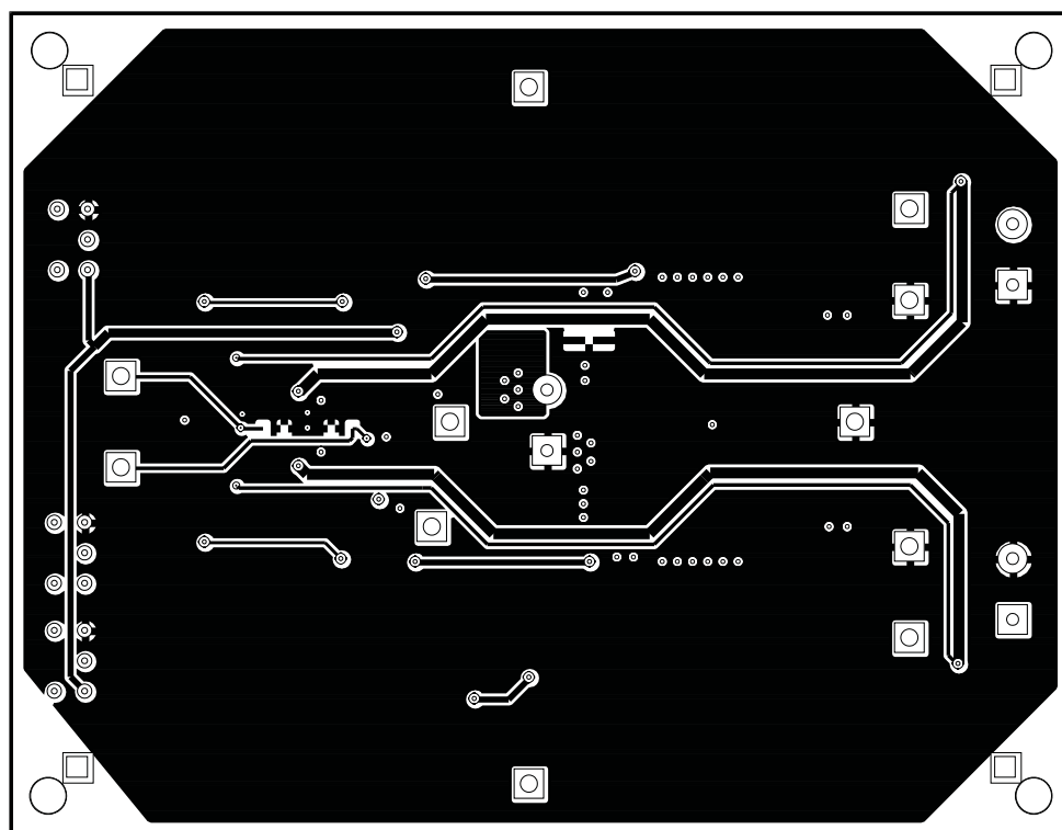
Figure 15. Bottom Layer
