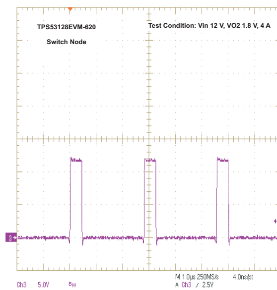
Figure 11. Switching Waveform
