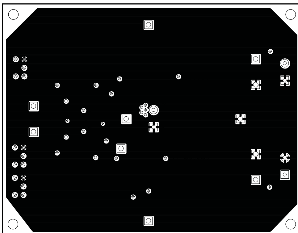
Figure 17. Internal Layer 2
