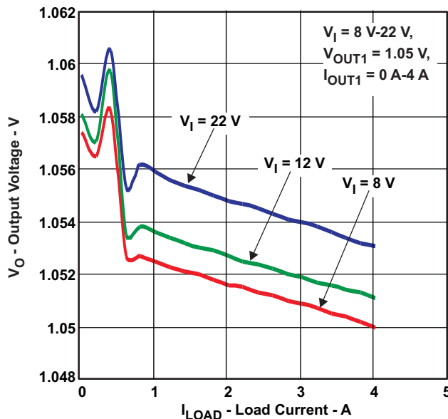
Figure 6. Output Voltage vs Load
