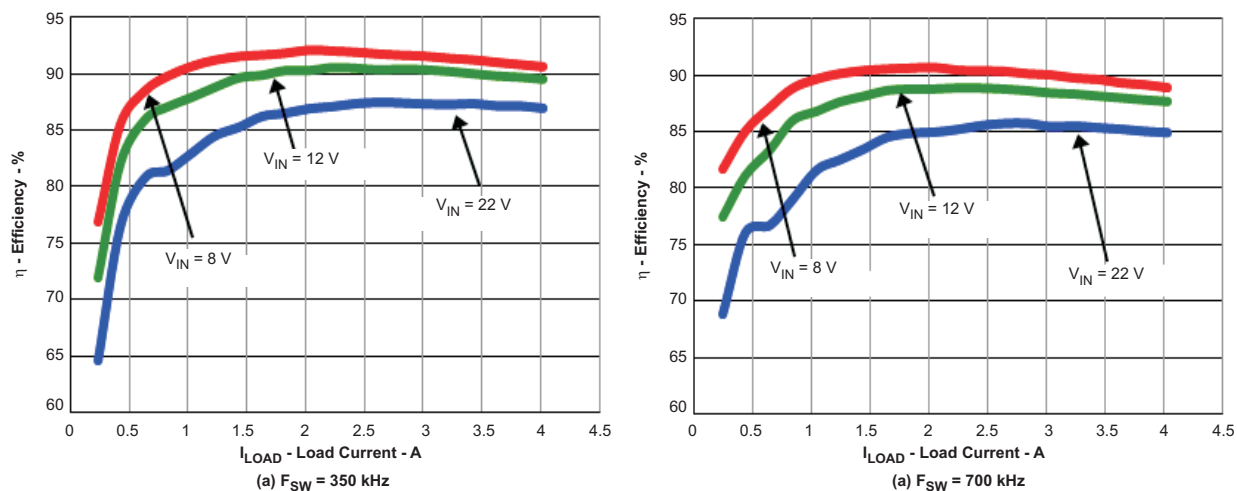
Figure 5. Efficiency vs Load ( V_{IN} = 8\text{ V} – 22\text{ V} , V_{OUT2} = 1.8\text{ V} , I_{OUT2} = 0\text{ A} – 4\text{ A} )
