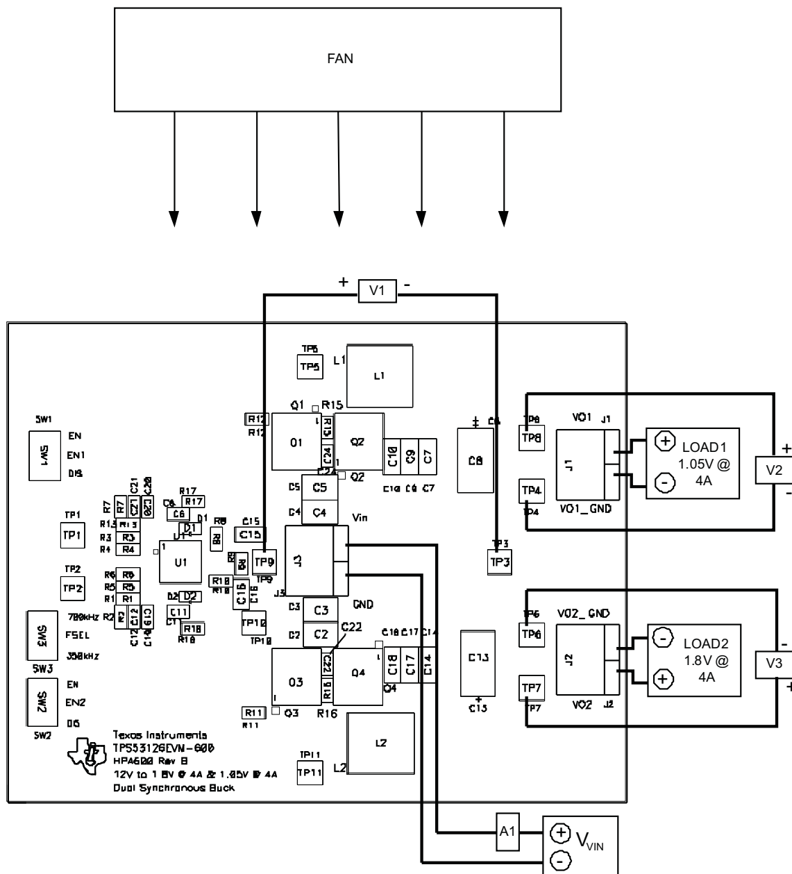
Figure 3. TPS53126EVM-600 Recommended Test Setup
