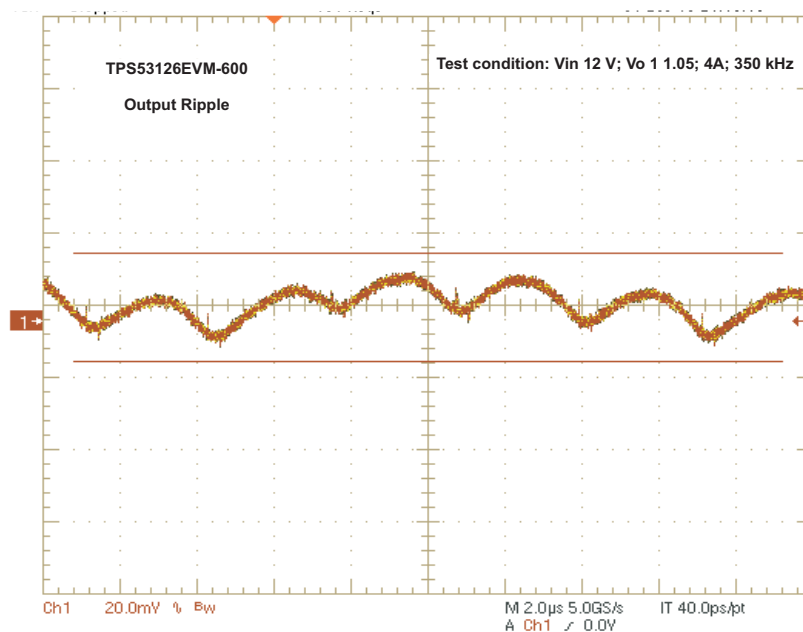
Figure 8. Output Voltage Ripple ( V_{IN} = 12 V, V_{OUT1} = 1.05 V, I_{OUT1} = 4 A, F_{SW} = 350 kHz)
