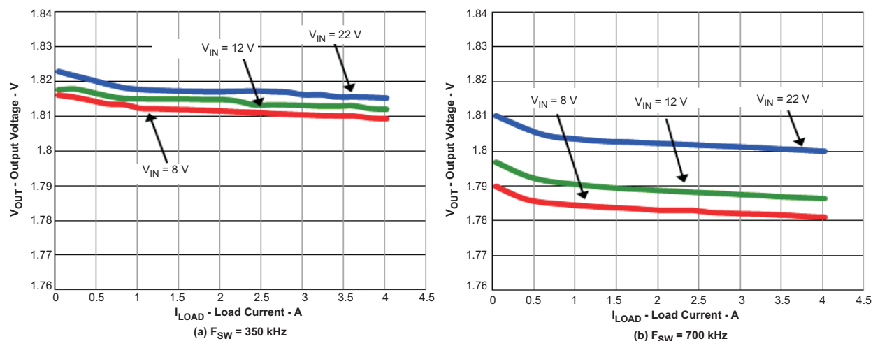
Figure 7. Output Voltage vs Load ( V_{IN} = 8 V–22 V, V_{OUT2} = 1.8 V, I_{OUT2} = 0 A–4 A)
