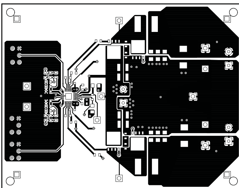
Figure 14. Top Layer
