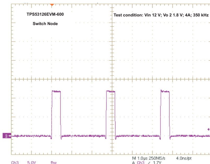
Figure 11. Switching Waveform ( V_{IN} = 12\text{ V} , V_{OUT2} = 1.08\text{ V} , I_{OUT2} = 4\text{ A} , F_{SW} = 350\text{ kHz} )
