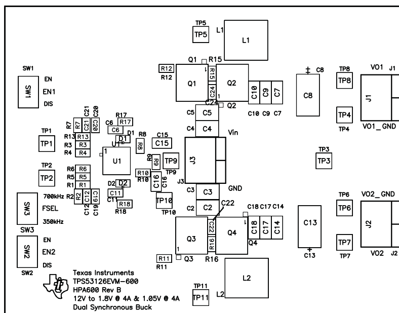
Figure 12. Top Assembly
