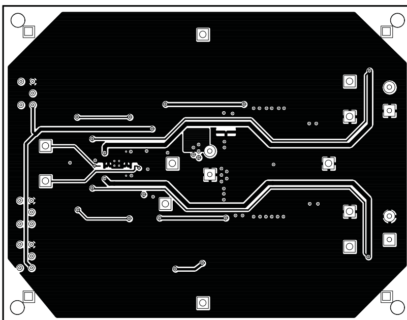
Figure 15. Bottom Layer
