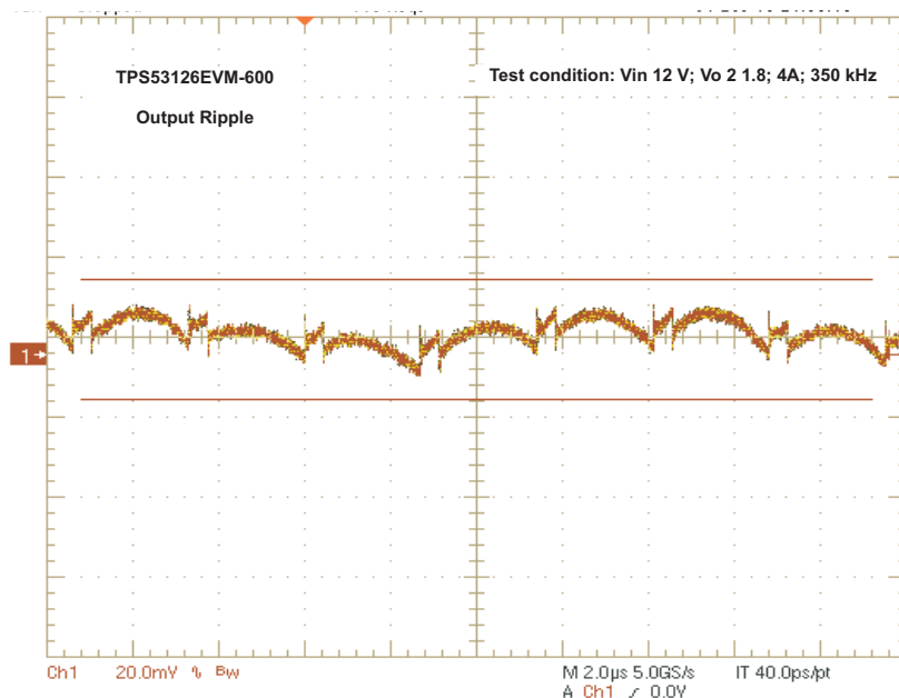
Figure 9. Output Voltage Ripple ( V_{IN} = 12\text{ V} , V_{OUT2} = 1.8\text{ V} , I_{OUT2} = 4\text{ A} , F_{SW} = 350\text{ kHz} )
