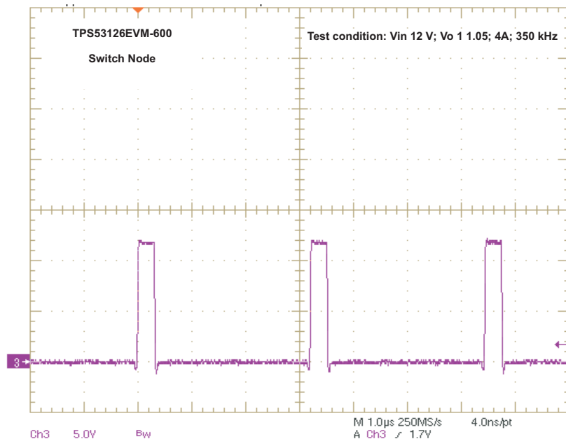
Figure 10. Switching Waveform ( V_{IN} = 12\text{ V} , V_{OUT1} = 1.05\text{ V} , I_{OUT1} = 4\text{ A} , F_{SW} = 350\text{ kHz} )
