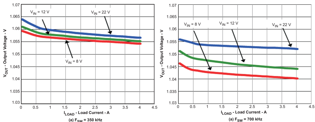
Figure 6. Output Voltage vs Load ( V_{IN} = 8\text{ V} – 22\text{ V} , V_{OUT1} = 1.05\text{ V} , I_{OUT1} = 0\text{ A} – 4\text{ A} )
