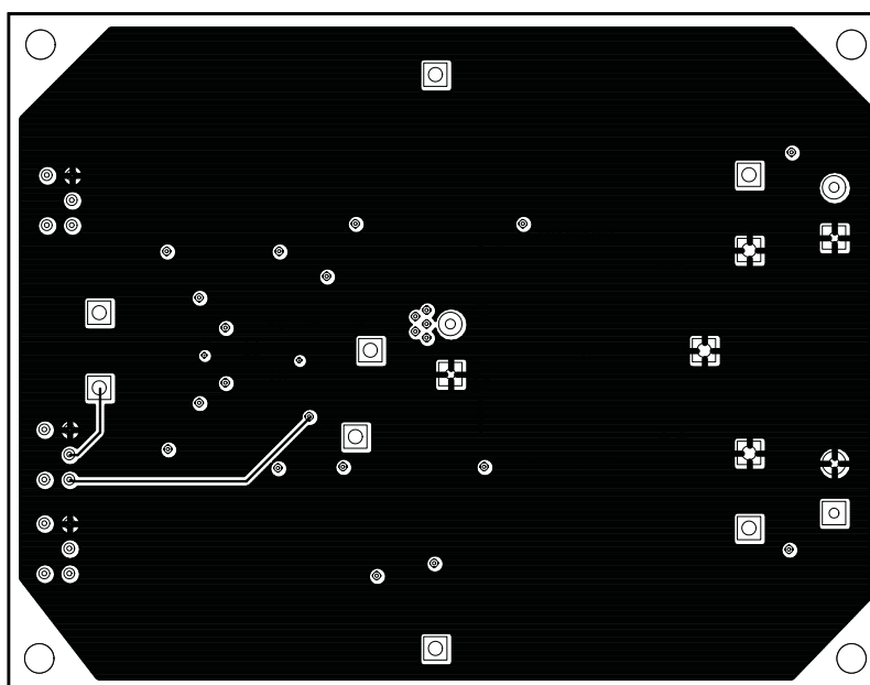
Figure 16. Internal Layer 1
