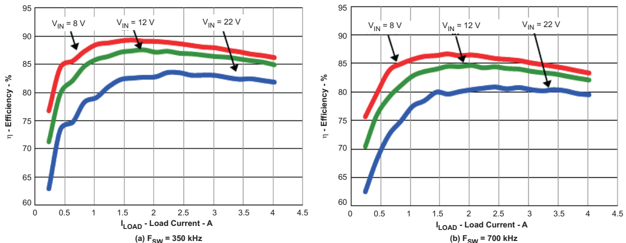
Figure 4. Efficiency vs Load ( V_{IN} = 8 V–22 V, V_{OUT1} = 1.05 V, I_{OUT1} = 0 A–4 A)
