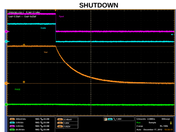
Figure 26. f = 800\text{kHz} , V_{\text{IN}} = 20\text{V} , I_{\text{OUT}} = 0\text{A}
