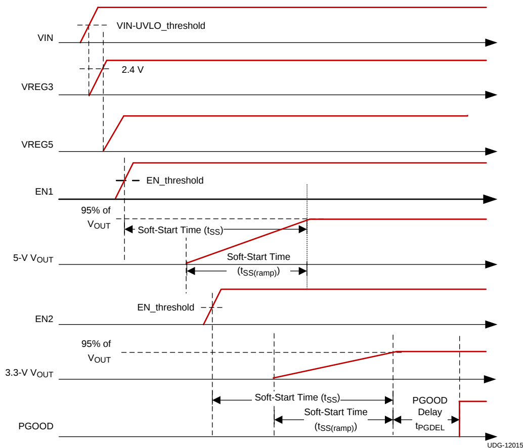
Figure 16. Timing Diagram
