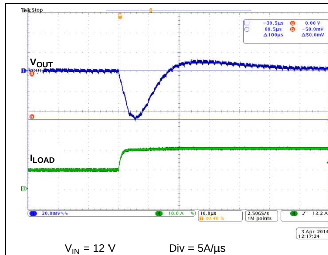
Figure 30. Load Step 10 A to 20 A
