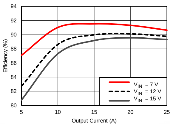
Figure 24. Efficiency vs Output Current
