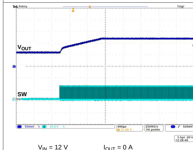
Figure 32. Prebias Sequence
