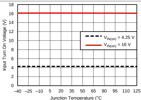
Figure 6. Input Turn-On Voltage vs. Junction Temperature
