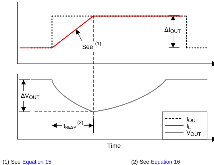
Figure 23. Load Transient Response Time
