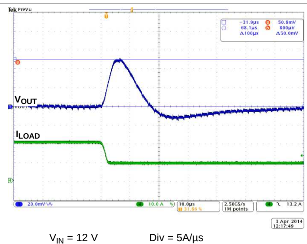
Figure 31. Load Step 20 A to 10 A
