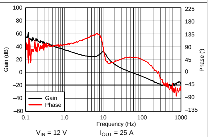
Figure 33. Bode Plot
