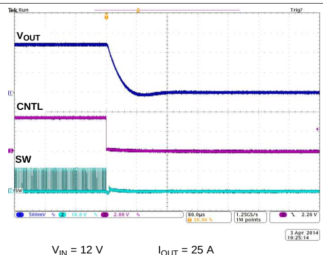
Figure 29. Shutdown from CNTL
