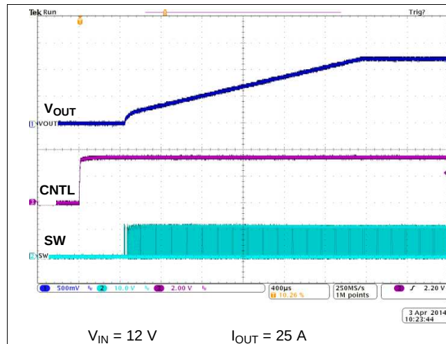
Figure 28. Startup from CNTL
