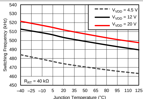
Figure 3. Switching Frequency vs Junction Temperature
