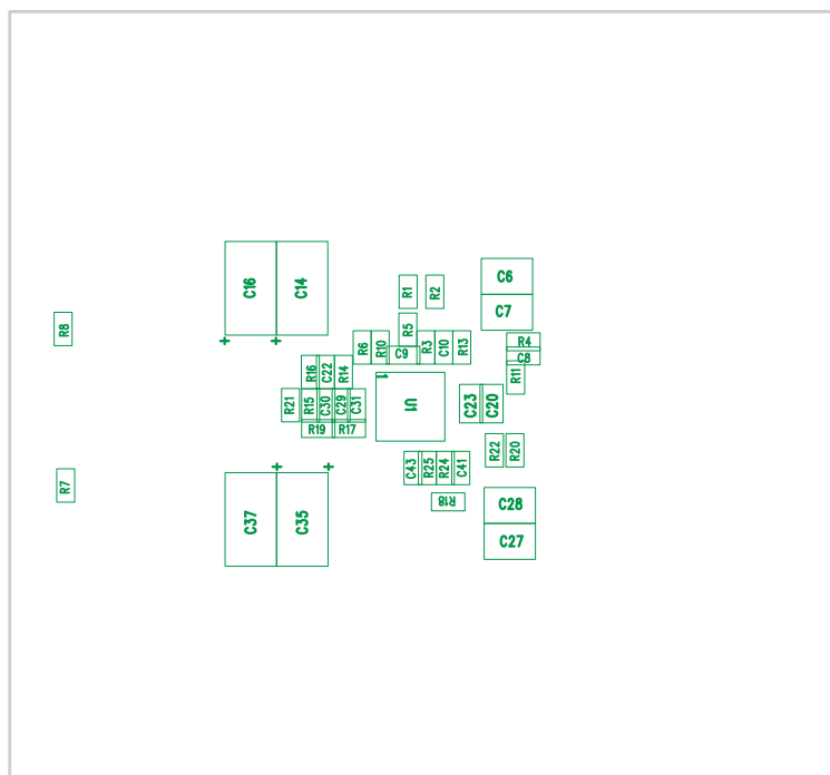
Figure 15. TPS40322EVM-074 Bottom Assembly Drawing (bottom view)
