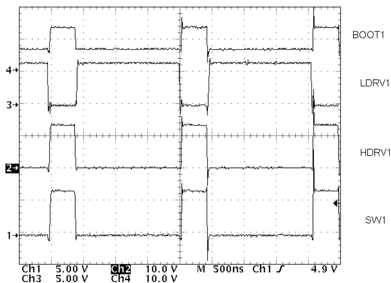
Figure 10. Switching Waveforms, (Ch1 = SW1, Ch2 = HDRV1, Ch3 = LDRV1, Ch4 = BOOT1, V_{IN} = 8\text{ V} , I_{OUT} = 30\text{ A} )
