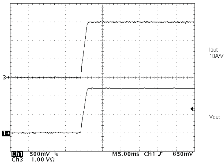
Figure 12. Enable turn on waveform, (Ch1 = V_{OUT} , Ch2 = I_{OUT} , V_{IN} = 8 V, I_{OUT} = 30 A (10 A/V scale))
