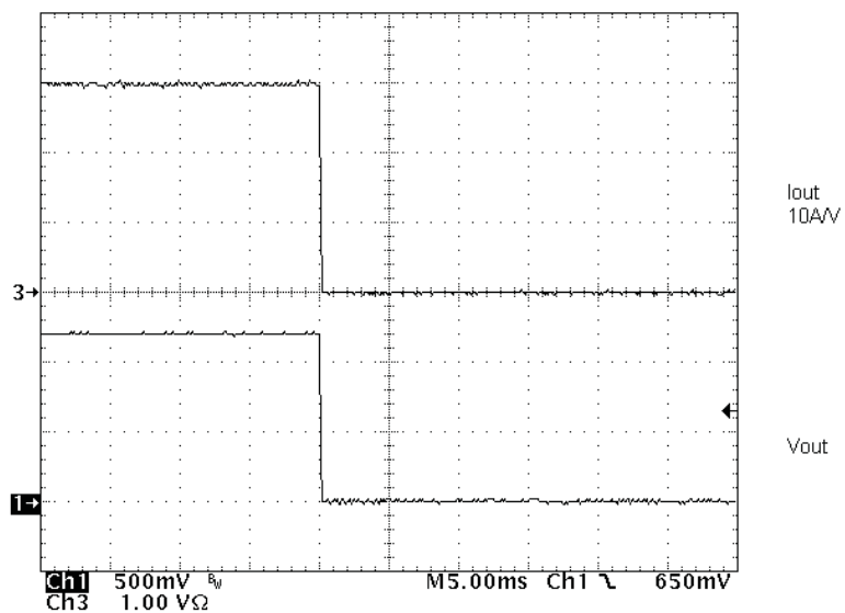
Figure 13. Enable turn off waveform, (Ch1 = V_{OUT} , Ch2 = I_{OUT} , V_{IN} = 8 V, I_{OUT} = 30 A (10 A/V scale))
