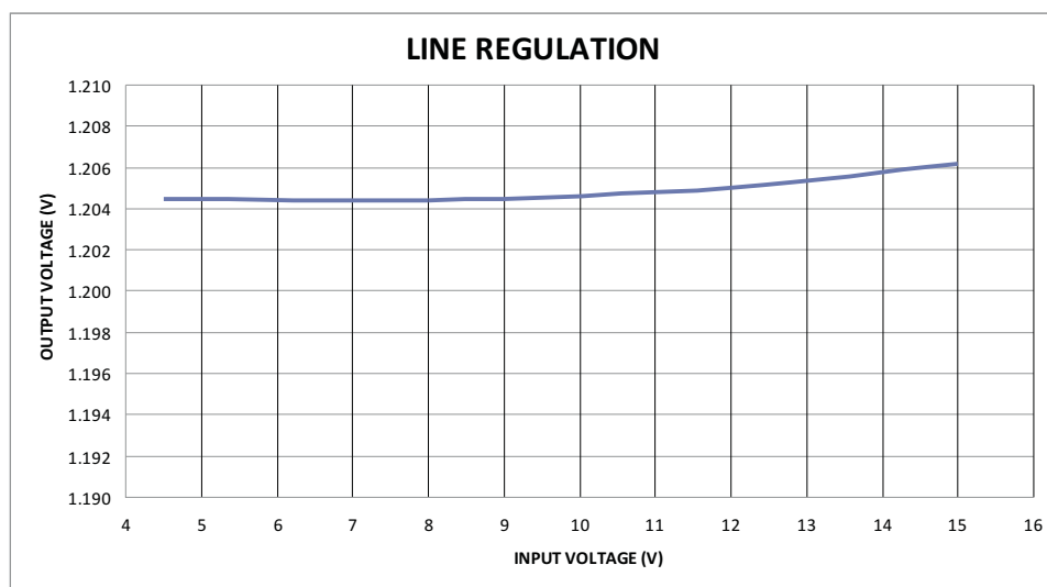
Figure 7. TPS40322EVM-074 Line Regulation
