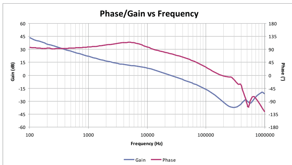
Figure 8. TPS40322EVM-074 Loop Response Gain and Phase ( V_{IN} = 8\text{ V} , I_{OUT} = 30\text{ A} , 76 degrees of phase margin at f_{CO} = 24\text{ kHz} )
