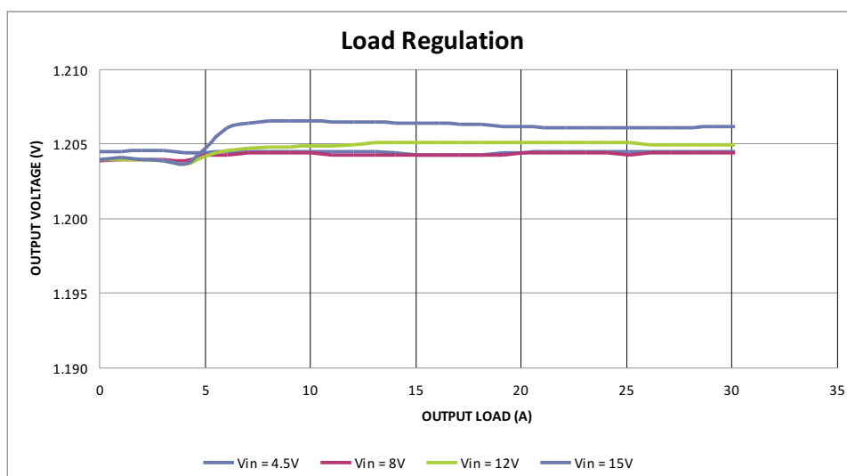
Figure 6. TPS40322EVM-074 Load Regulation
