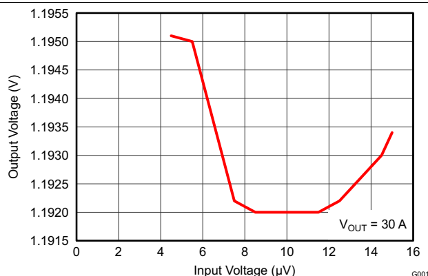
Figure 31. Line Regulation
