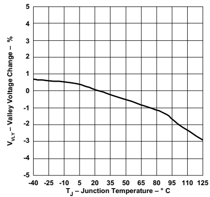
Figure 16. Valley Voltage Change vs Junction Temperature
