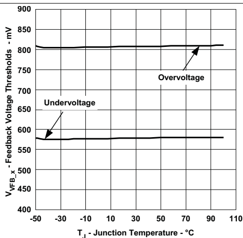
Figure 13. Undervoltage and Overvoltage Threshold vs Junction Temperature
