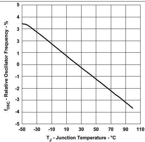
Figure 19. Relative Oscillator Frequency vs Junction Temperature
