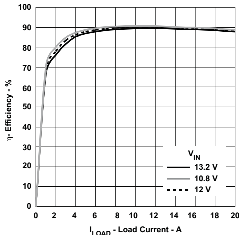
Figure 34. Efficiency Curve
