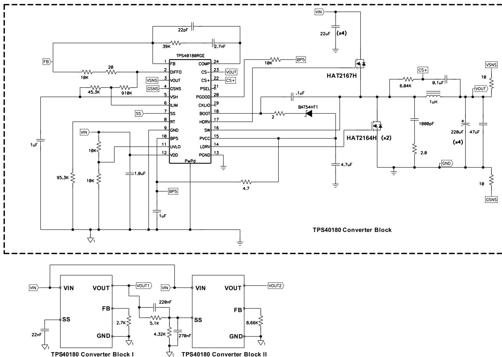
Figure 36. Simultaneous Tracking With TPS40180
