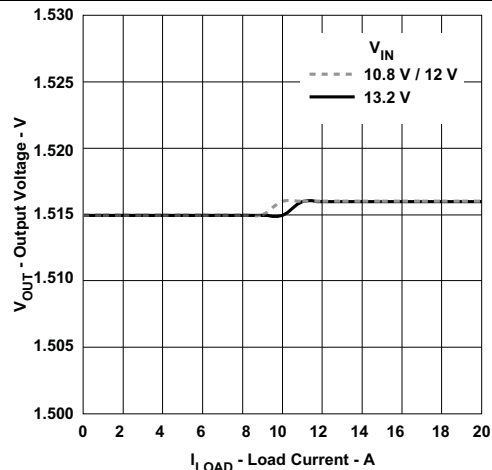
Figure 35. Output Load Regulation
