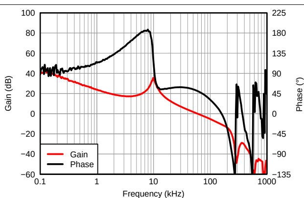
Figure 37. Loop Response
