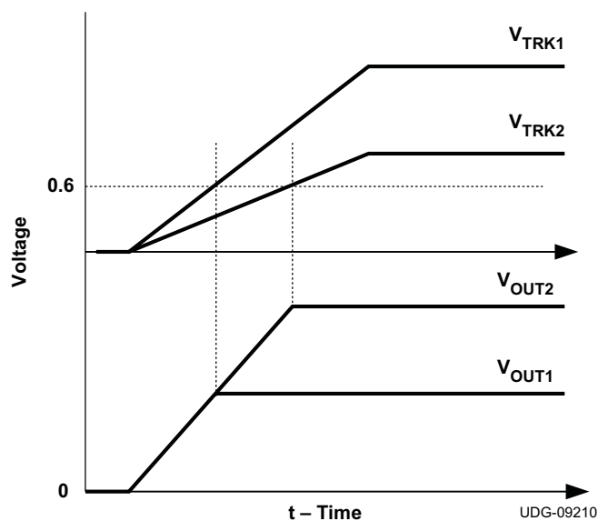
Figure 26. Simultaneous Voltage Tracking Waveform
