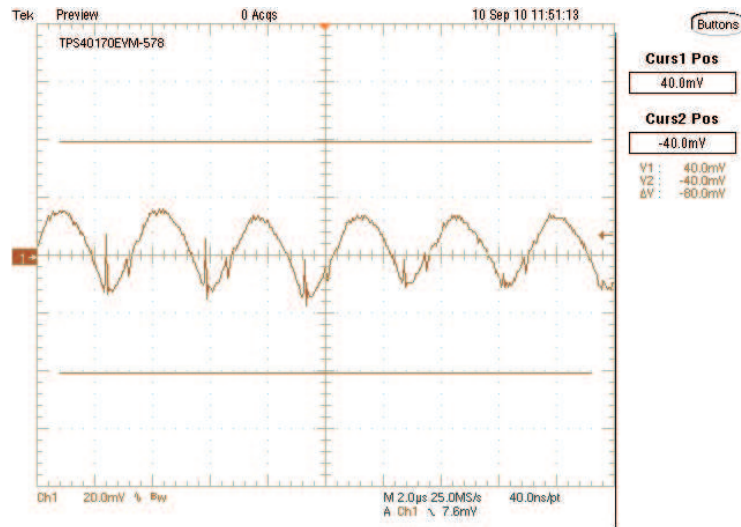
Figure 38. Output Ripple Waveform
