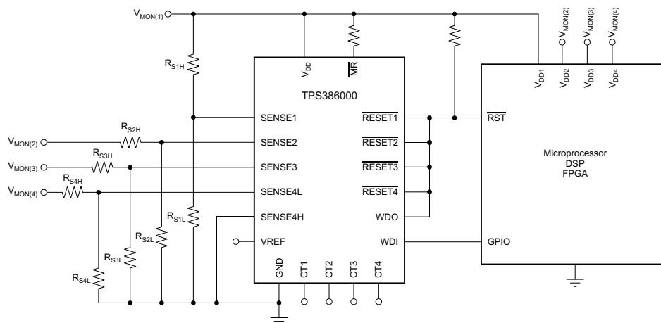
TPS386000 Typical Application Circuit: Monitoring Supplies for an FPGA
