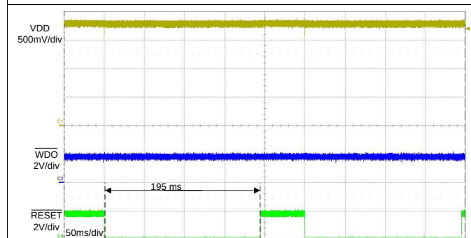
Figure 30. Typical RESET Delay
