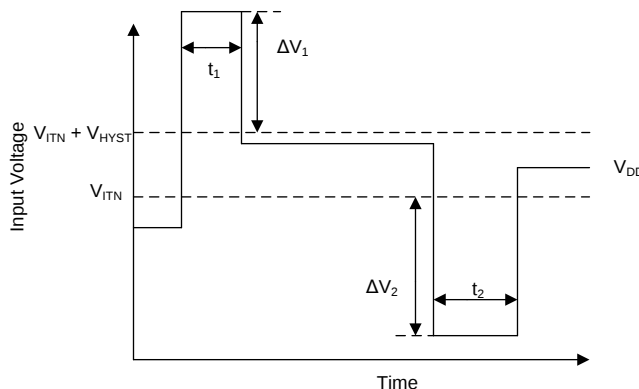
Figure 25. Overdrive Voltage
