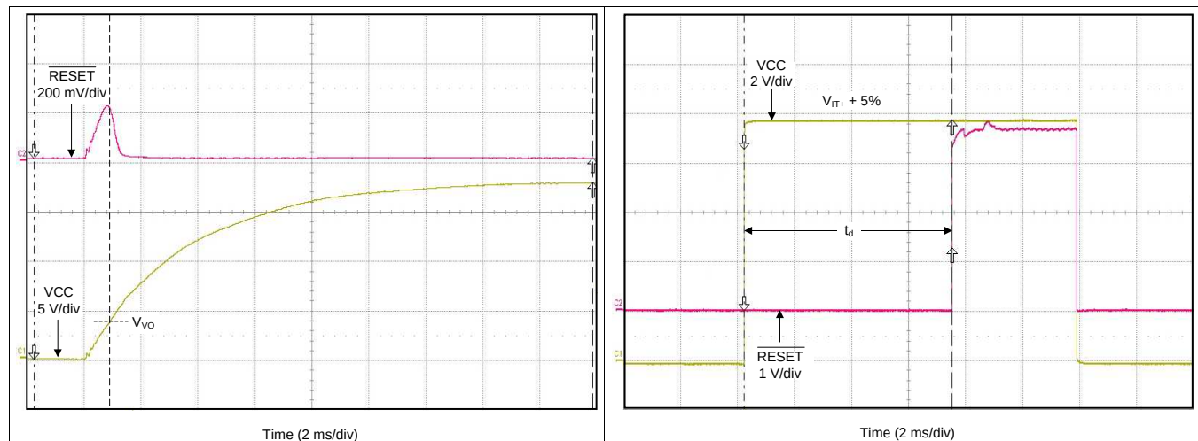
Figure 17. Startup Showing Minimum V_{(VCC)} for Valid Output
