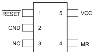
Pin Functions
