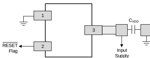
Figure 18. Recommended Layout
