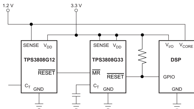
Typical Application
