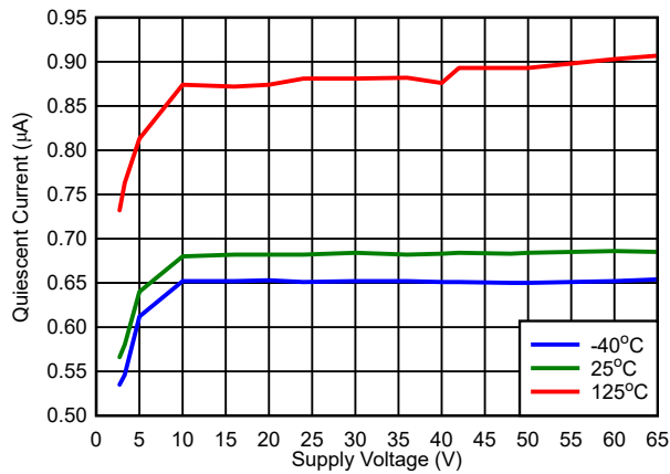
Figure 7-3. V_{DD} vs I_{DD} ( \overline{\text{RESET}} = High, V_{IT} = 2.7\text{ V} )
