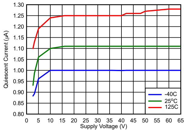
Figure 7-5. V_{DD} vs I_{DD} ( \overline{\text{RESET}} = High, V_{IT} = 0.8\text{ V} )
