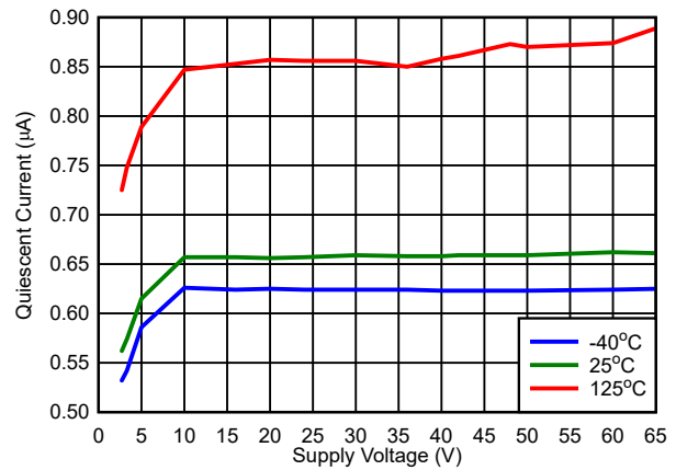
Figure 7-4. V_{DD} vs I_{DD} ( \overline{\text{RESET}} = Low, V_{IT} = 2.7\text{ V} )
