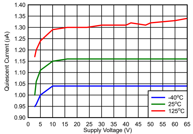
Figure 7-6. V_{DD} vs I_{DD} ( \overline{\text{RESET}} = Low, V_{IT} = 0.8\text{ V} )
