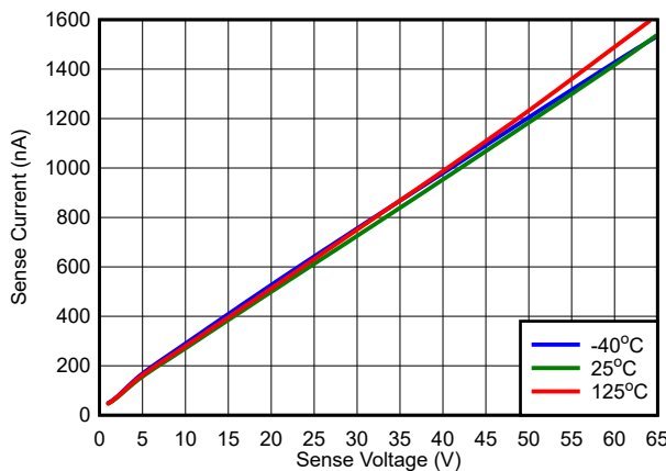
Figure 7-7. V_{SENSE} vs I_{SENSE} V_{DD} = 2.7\text{ V}
