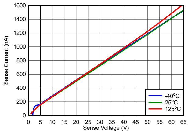
Figure 7-8. V_{SENSE} vs I_{SENSE} V_{DD} = 65\text{ V}
