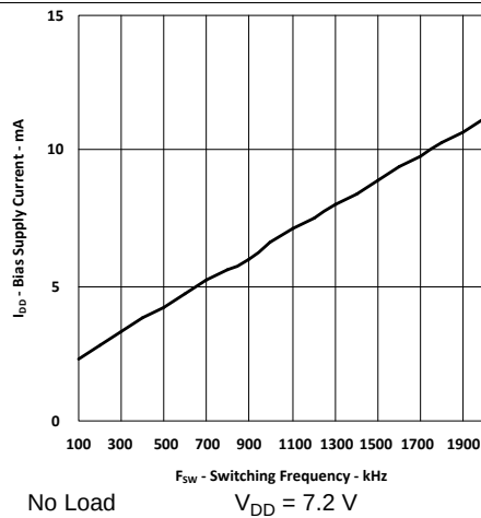
Figure 14. Bias Supply Current vs Switching Frequency
