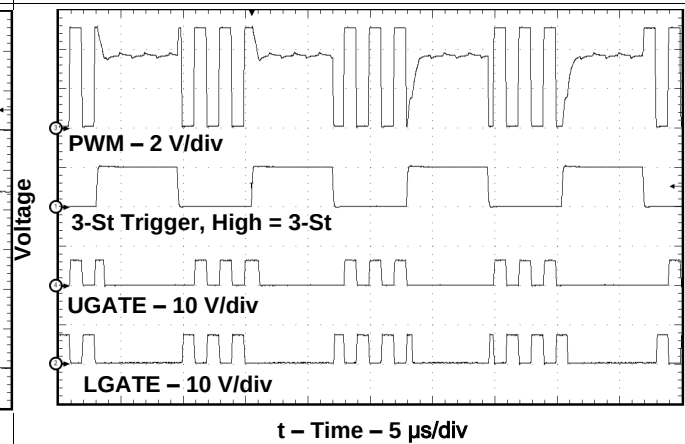
Figure 17. PWM Input Falling Switching Waveforms
