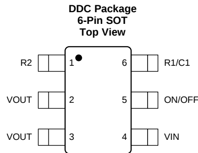
Pin Functions
