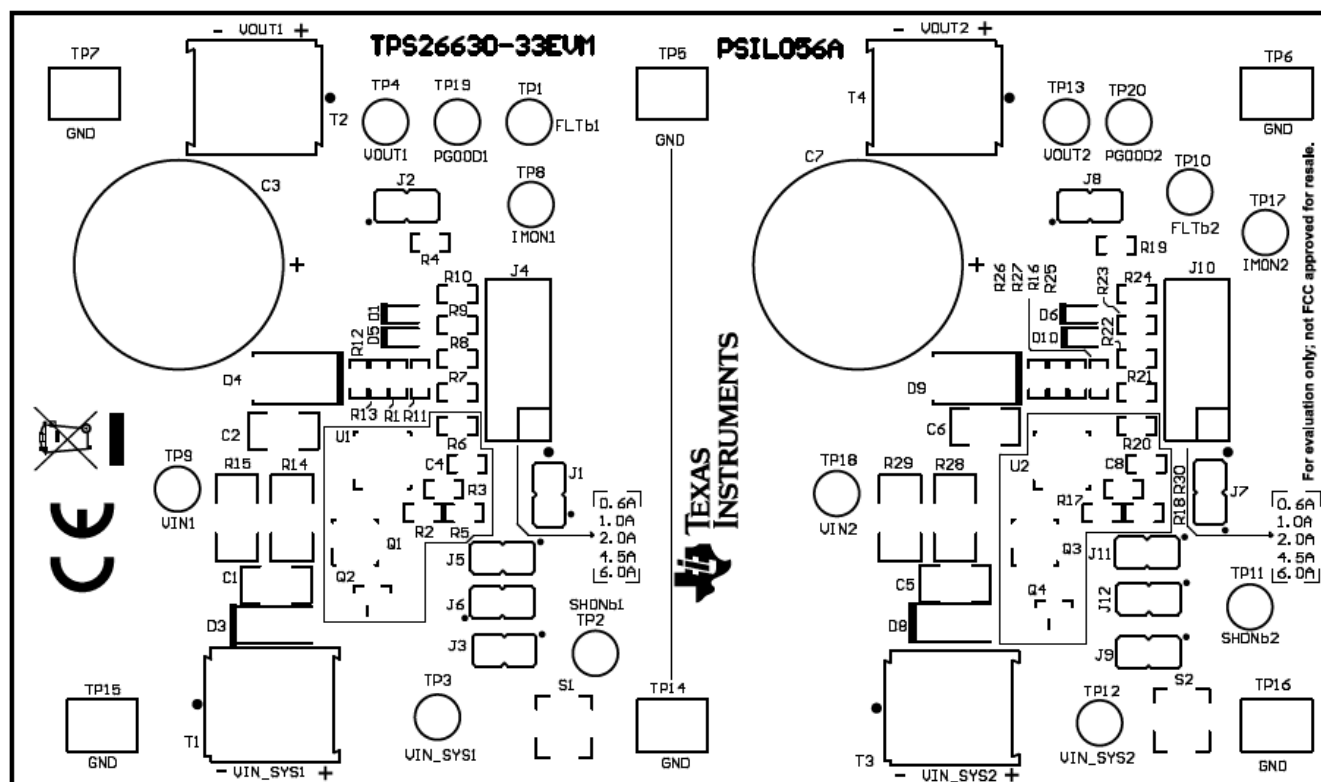
Figure 8. Top Side Placement
