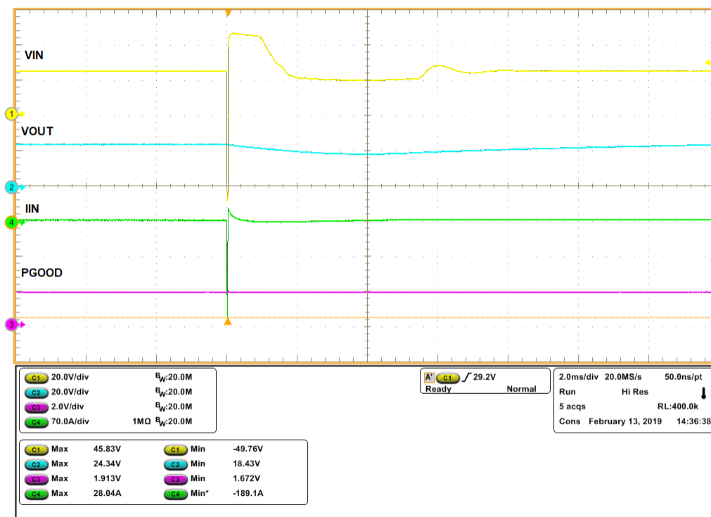
Figure 5. -500-V Surge Protection [ C_{OUT} = 2 \text{ mF} , R_{LOAD} = 6 \Omega , V_{IN} = 24 \text{ V} , I_{LIM} = 4.5 \text{ A} , Peak Pulse Power = 9.4 kW]
