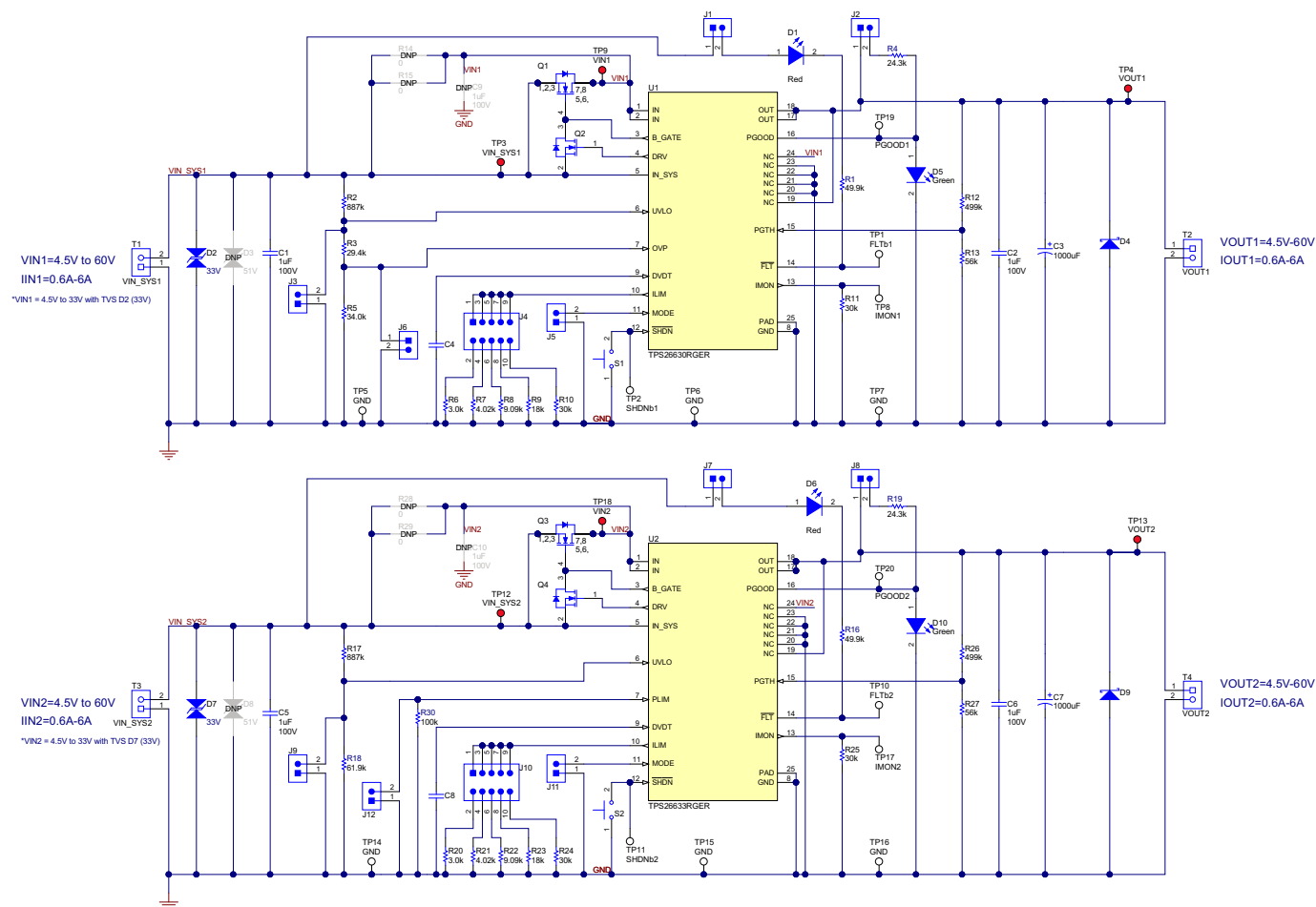
Figure 11. TPS26630-33EVM Schematic
