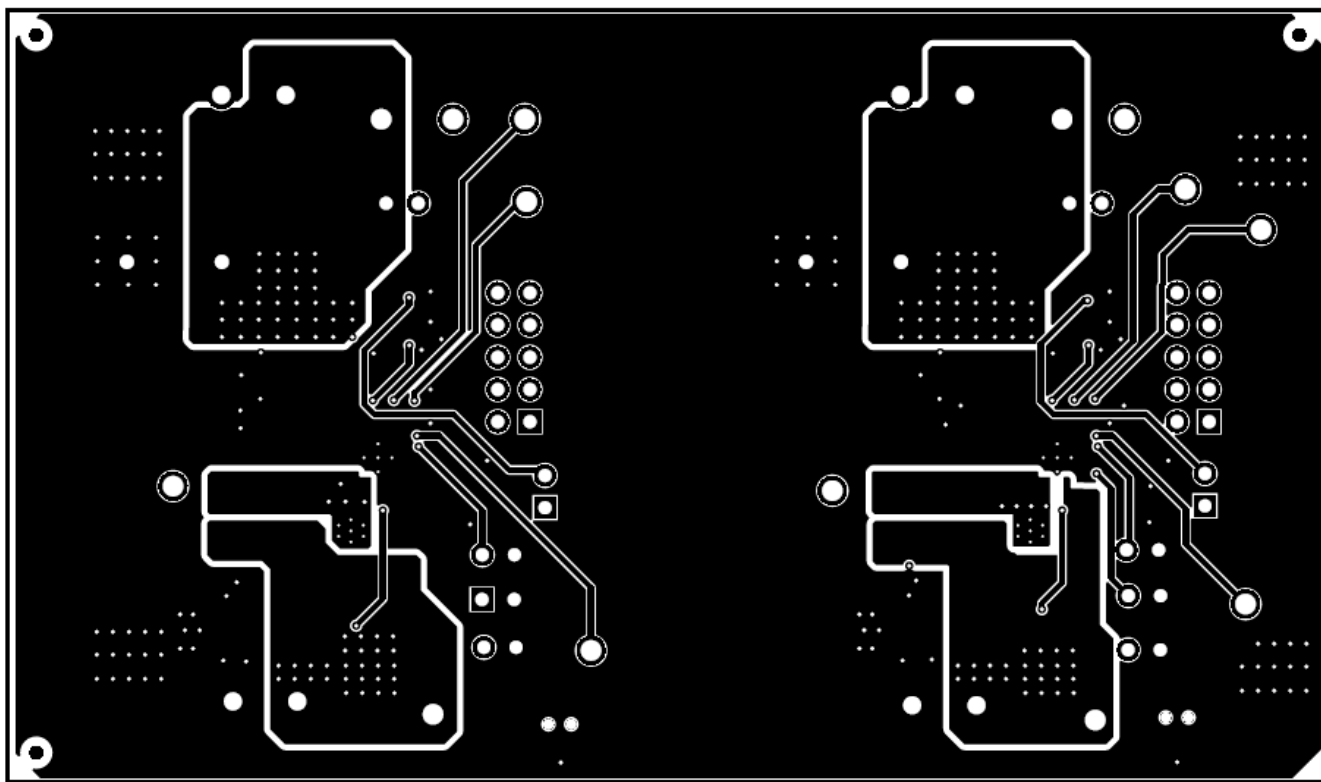
Figure 10. Bottom Layer
