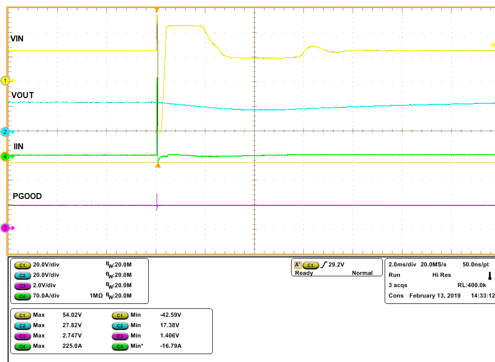
Figure 4. +500-V Surge Protection [ C_{\text{OUT}} = 2\text{ mF} , R_{\text{LOAD}} = 6\text{ }\Omega , V_{\text{IN}} = 24\text{ V} , I_{\text{LIM}} = 4.5\text{ A} , Peak Pulse Power = 12 kW]
