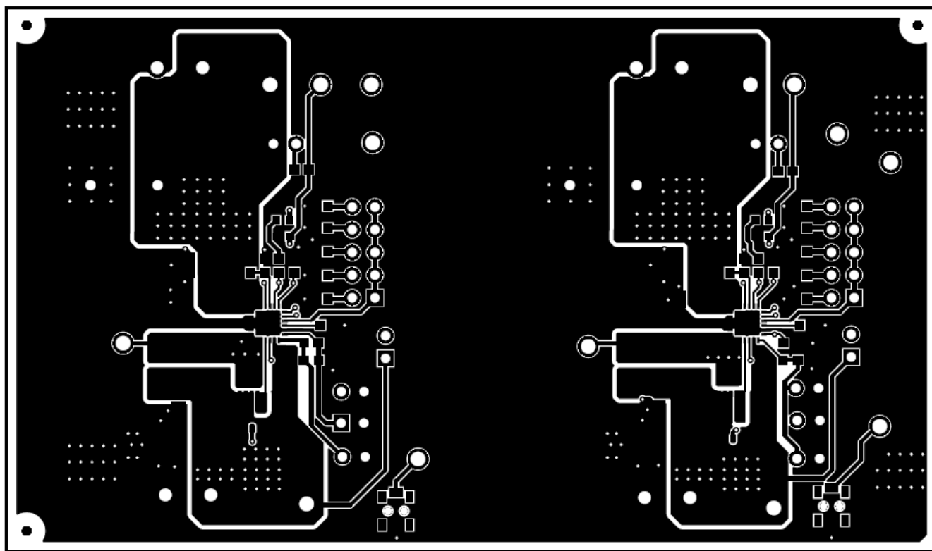
Figure 9. Top Layer
