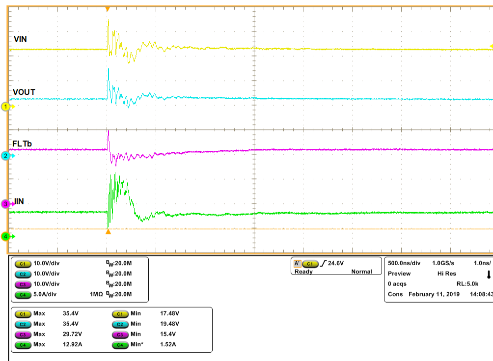
Figure 6. +2-kV EFT Protection [ C_{OUT} = 1 \mu F , R_{LOAD} = 4.8\text{-}\Omega , V_{IN} = 24\text{ V} , I_{LIM} = 6\text{ A} ]
