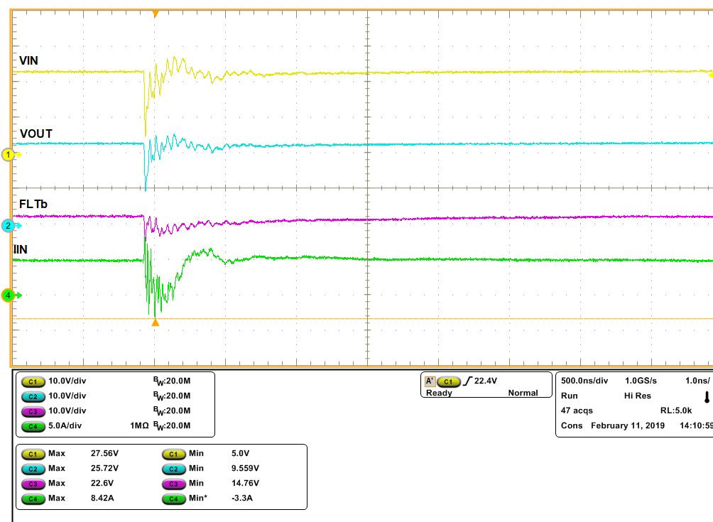
Figure 7. -2-kV EFT Protection [ C_{OUT} = 1 \mu F , R_{LOAD} = 4.8\text{ }\Omega , V_{IN} = 24\text{ V} , I_{LIM} = 6\text{ A} ]
