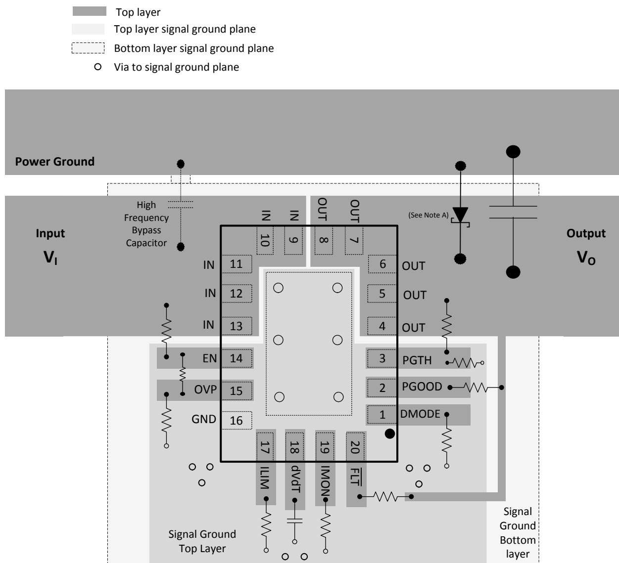
Figure 88. Board Layout
