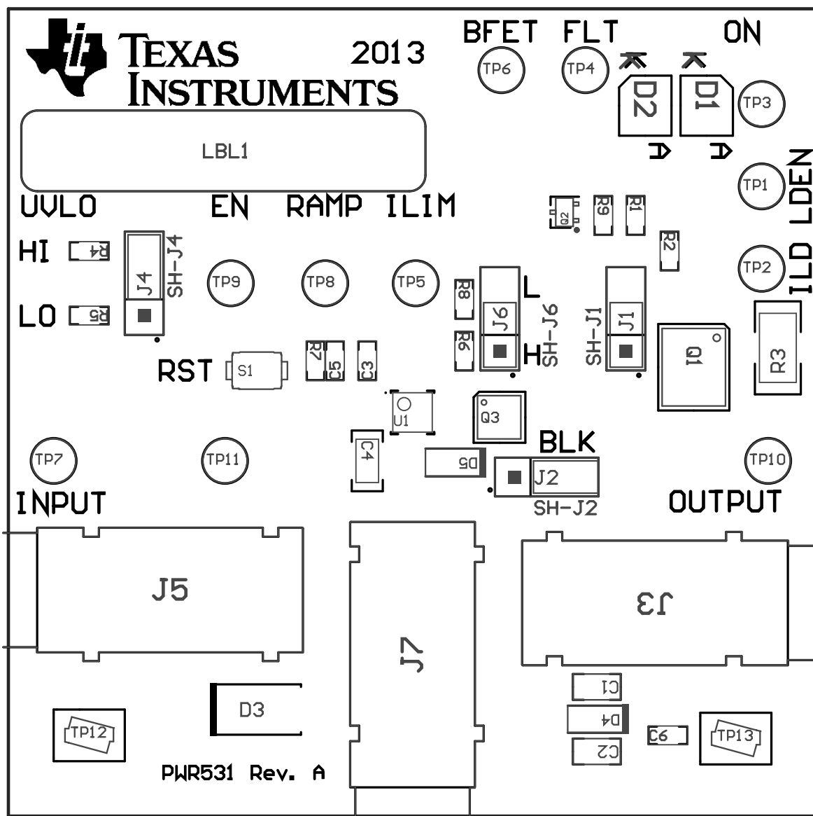
Figure 4-1. Top-Side Placement
