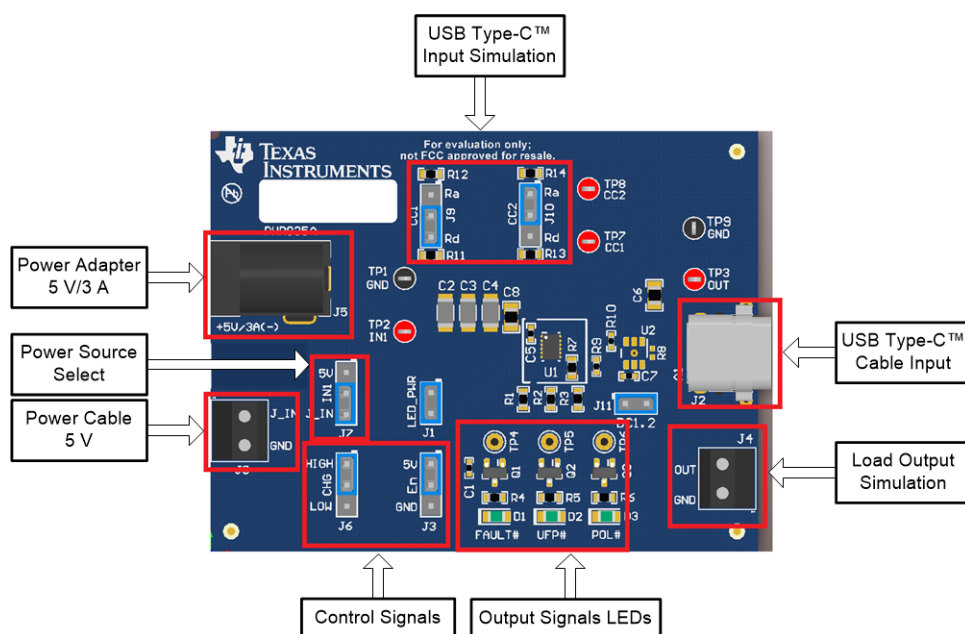
Figure 1. TPS25820/21EVM
