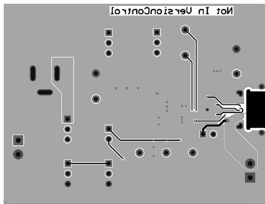
Figure 15. Bottom Layer
