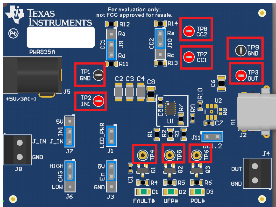
Figure 3. Test Points
