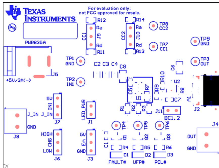
Figure 12. Top Silkscreen
