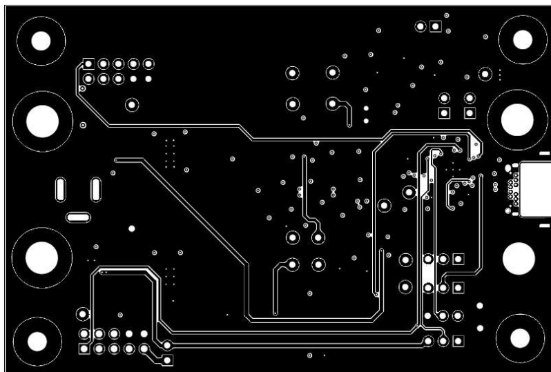
Figure 27. Signal Layer 2
