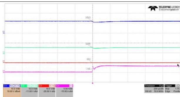
Figure 16. Load Step From 0 A to 3 A (12 V)
