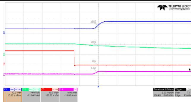
Figure 10. 5-V to 12-V Transition
