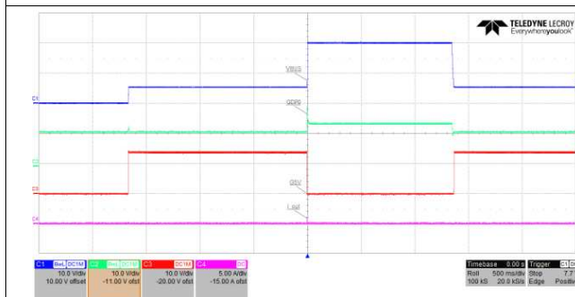
Figure 8. Mux Between 5 V and 20 V at No Load
