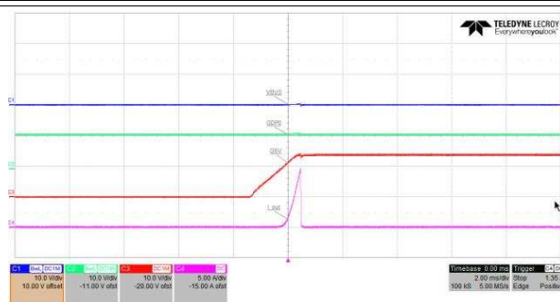
Figure 12. Start Into Short on Output
