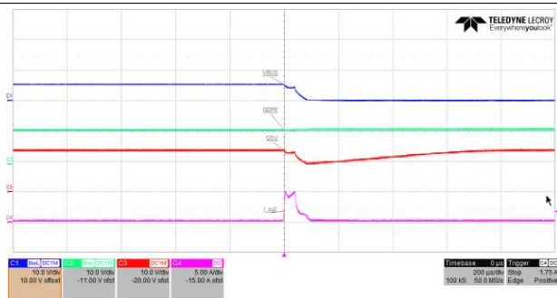
Figure 18. 5.5-A Load Step Triggers OCP (5 V)
