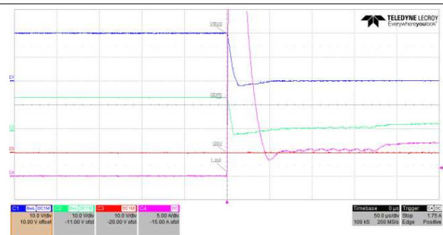
Figure 15. Hot Short on Output 20 V
