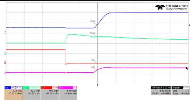
Figure 11. 5-V to 20-V Transition
