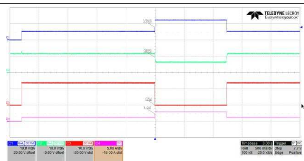
Figure 7. Mux Between 5 V and 12 V at 3 A
