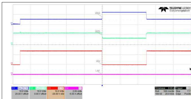
Figure 6. Mux Between 5 V and 12 V at No Load
