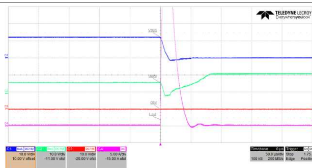
Figure 14. Hot Short on Output 12 V
