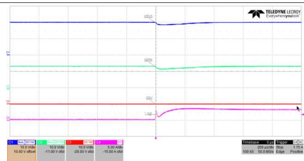
Figure 17. Load Step From 0 A to 3 A (20 V)
