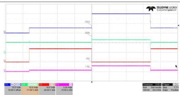
Figure 9. Mux Between 5 V and 20 V at 3 A
