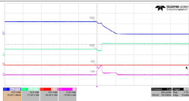
Figure 19. 5.5-A Load Step Triggers OCP (12 V)
