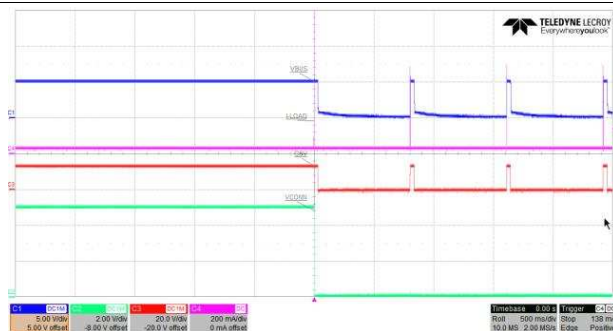
Figure 23. VCONN OCP
