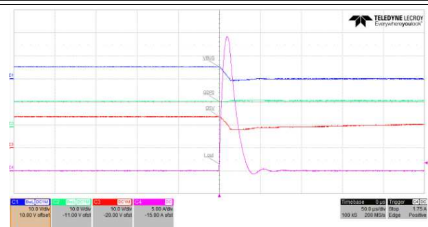
Figure 13. Hot Short on Output 5 V
