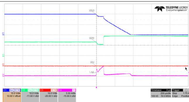
Figure 20. 5.5-A Load Step Triggers OCP (20 V)
