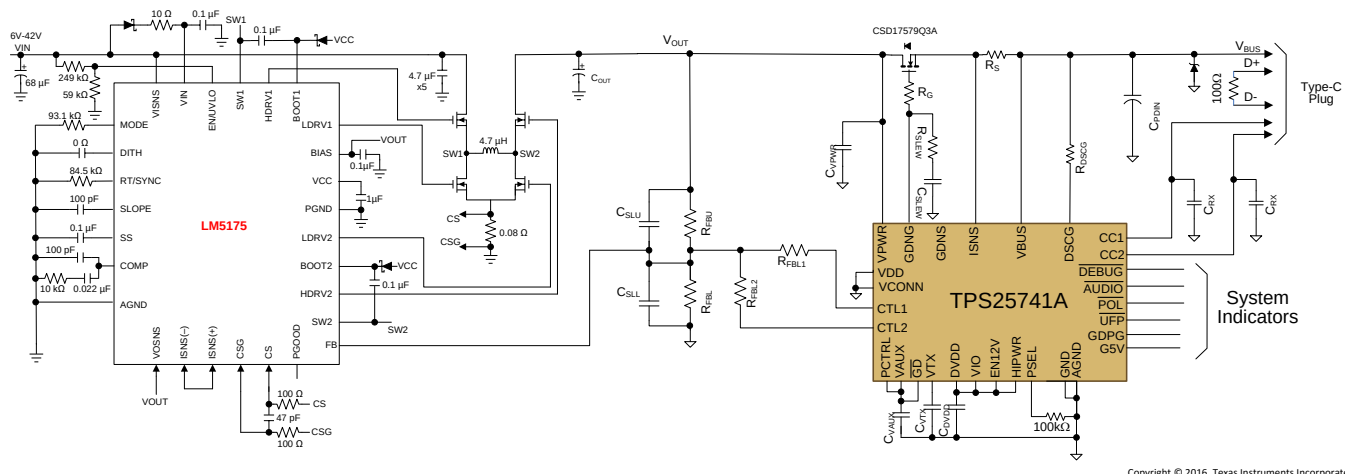
Figure 64. DC Power Source
