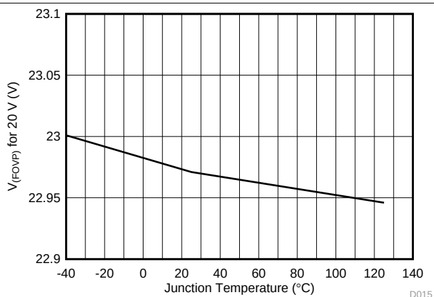
Figure 14. V FOVP While Supplying 20 V, TPS25741
