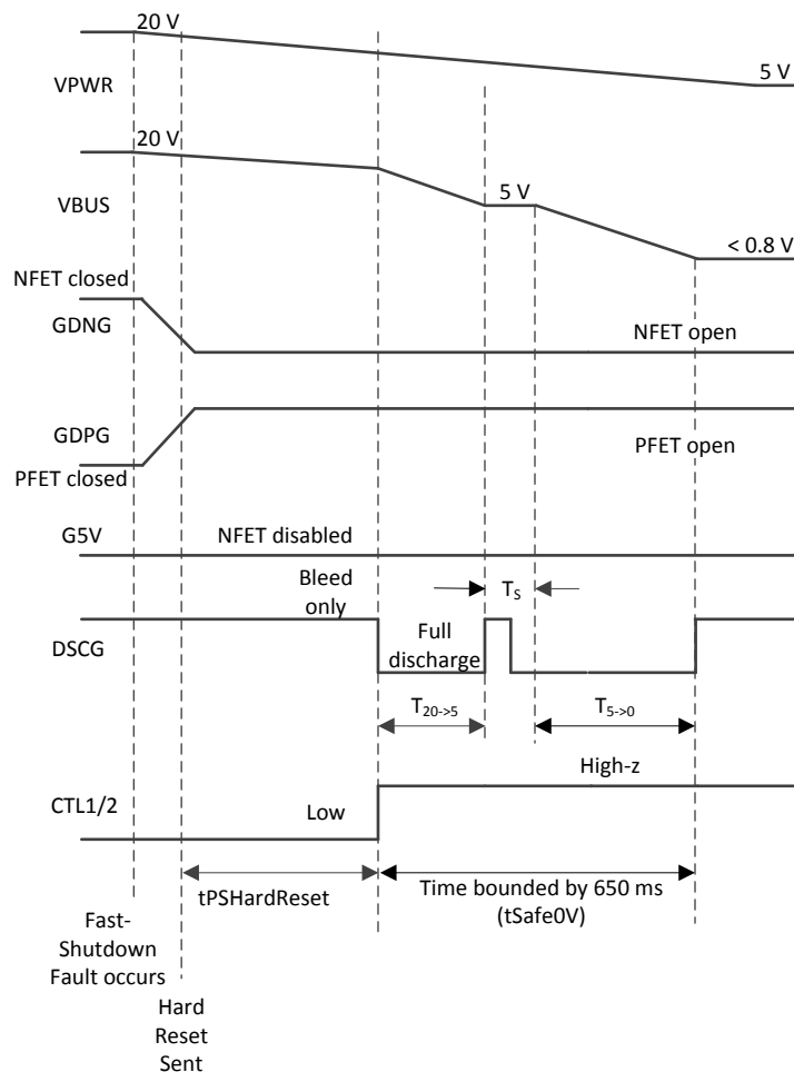
Figure 33. Illustration of Fast-Shutdown Discharge
