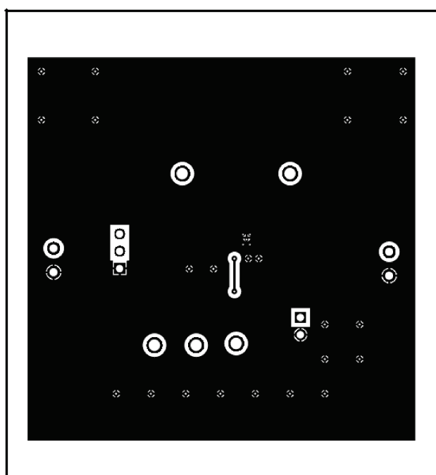
Figure 5. Bottom Side Routing
