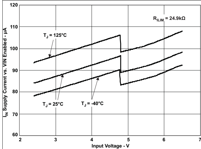
Figure 9. Supply Current, Output Enabled
