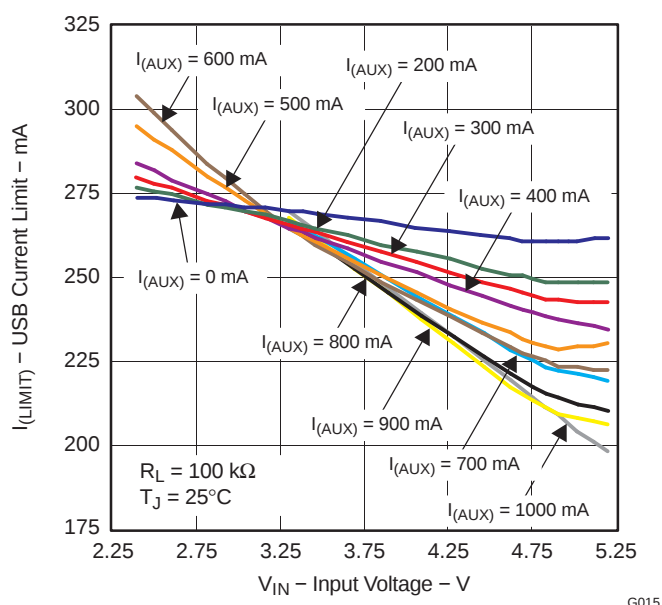
Figure 19. USB Current-Limit Threshold vs V_{IN} , R_{ILIM} = 100\text{ k}\Omega , T_A = 25^\circ\text{C}
