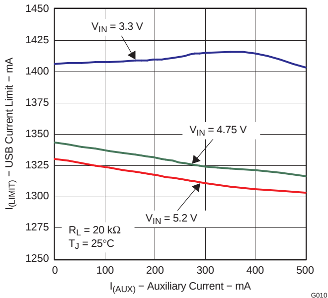
Figure 14. USB Current-Limit Threshold vs I_{AUX} , R_{ILIM} = 20\text{ k}\Omega , T_A = 25^\circ\text{C}
