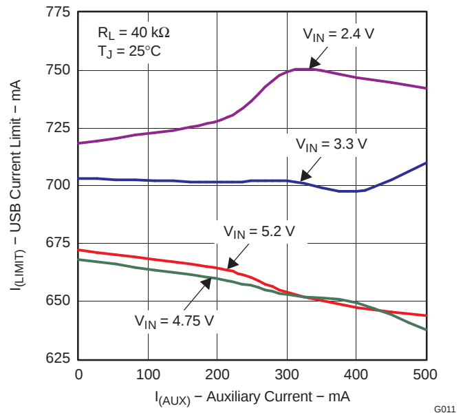
Figure 15. USB Current-Limit Threshold vs I_{AUX} , R_{ILIM} = 40\text{ k}\Omega , T_A = 25^\circ\text{C}
