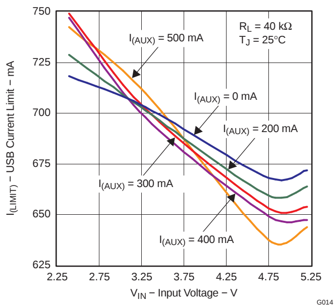
Figure 18. USB Current-Limit Threshold vs V_{IN} , R_{ILIM} = 40\text{ k}\Omega , T_A = 25^\circ\text{C}
