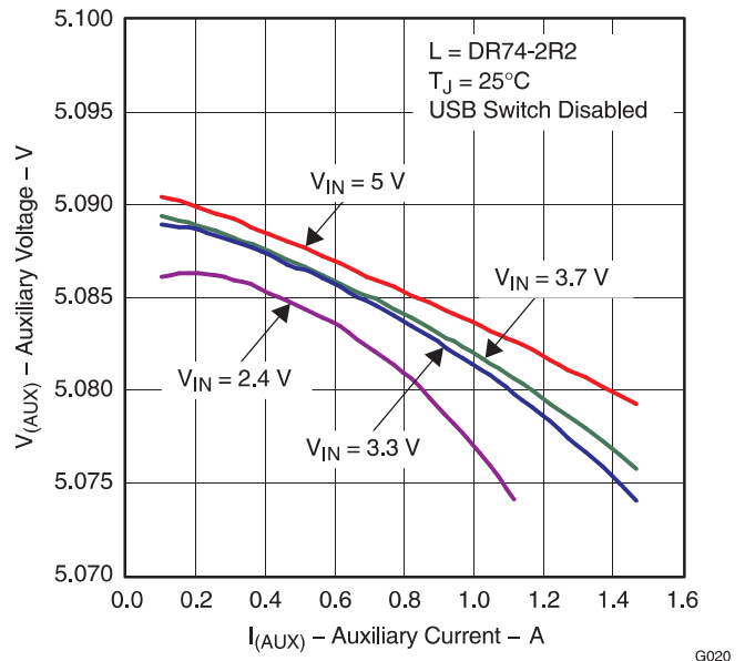
Figure 27. Load Regulation, TPS2501 (Forced PWM Mode)
