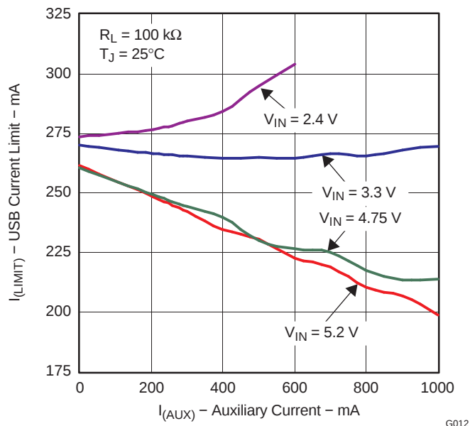
Figure 16. USB Current-Limit Threshold vs I_{AUX} , R_{ILIM} = 100\text{ k}\Omega , T_A = 25^\circ\text{C}
