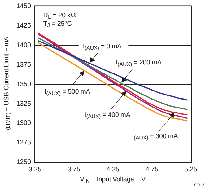
Figure 17. USB Current-Limit Threshold vs V_{IN} , R_{ILIM} = 20\text{ k}\Omega , T_A = 25^\circ\text{C}
