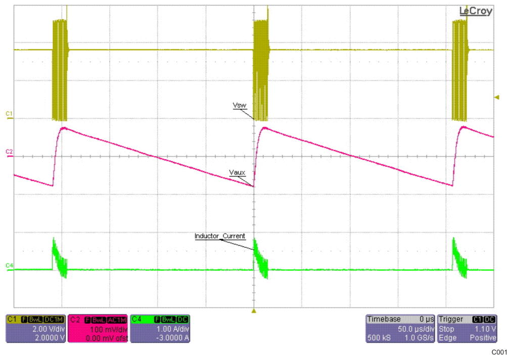
Figure 11. Eco-mode Control Scheme Operation, V_{IN} = 3.3 V, I_{AUX} = 10 mA
