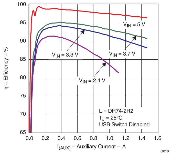
Figure 25. Efficiency vs I_{AUX} , TPS2501 (Forced PWM Mode)
