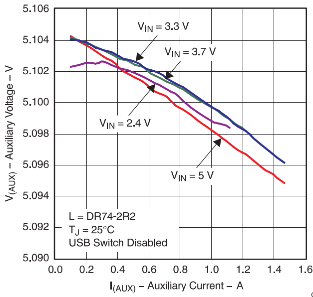
Figure 26. Load Regulation, TPS2500 (Eco-mode Control Scheme)
