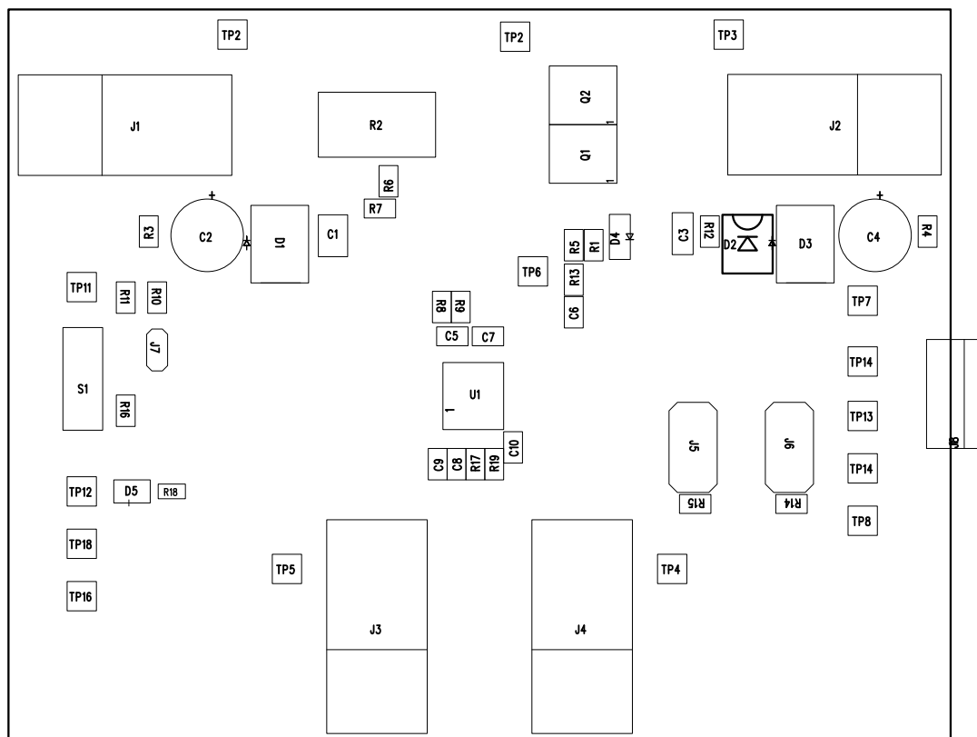
Figure 6. Top Assembly
