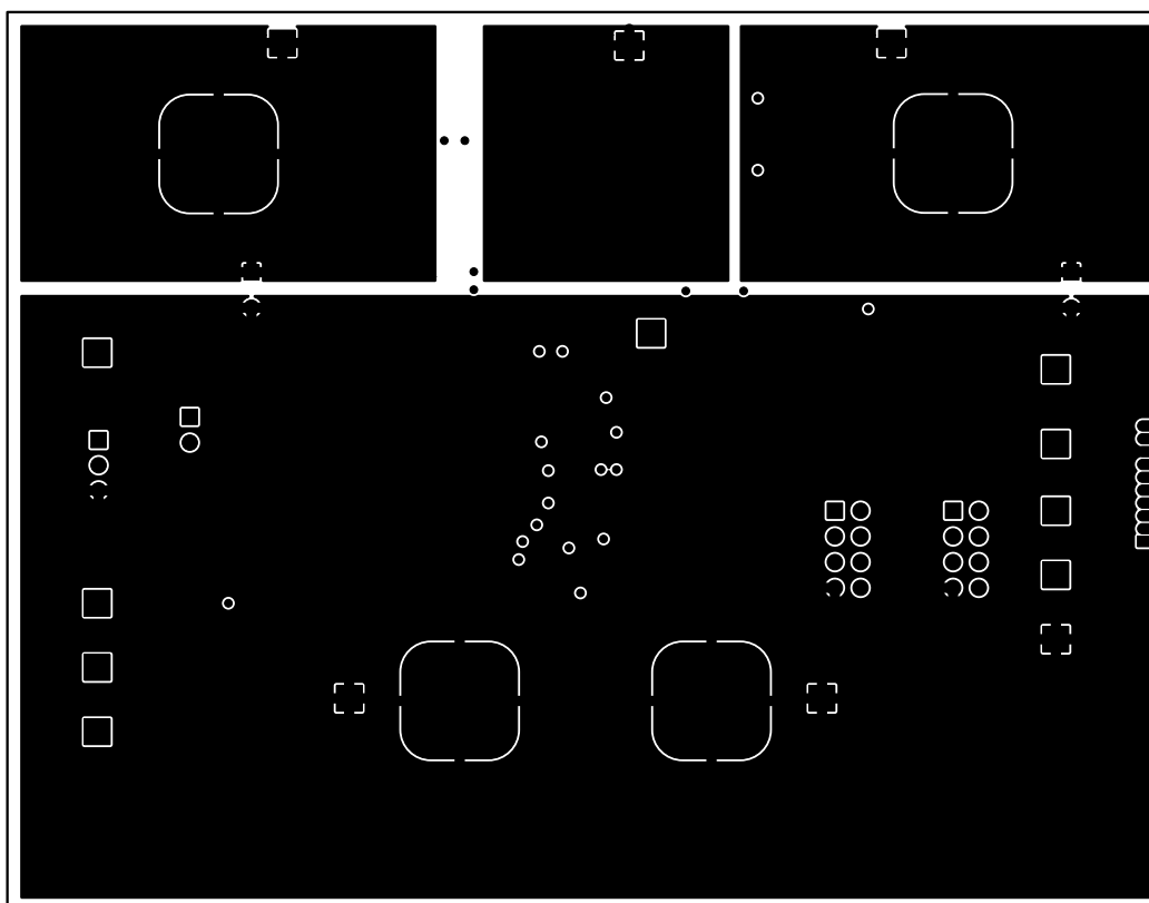
Figure 10. Bottom Layout
