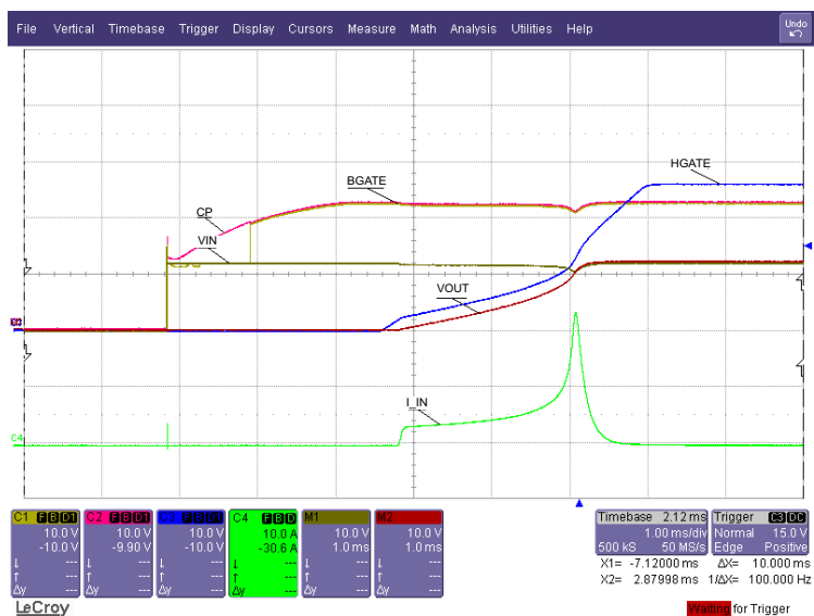
Figure 7. Startup ( C_O = 440 \mu F )
