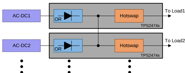
Figure 1. Block Diagram for Systems With Multiple Supplies and Loads
