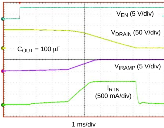
Figure 5. Start-up from Enable, V_{IN} = -80 V
