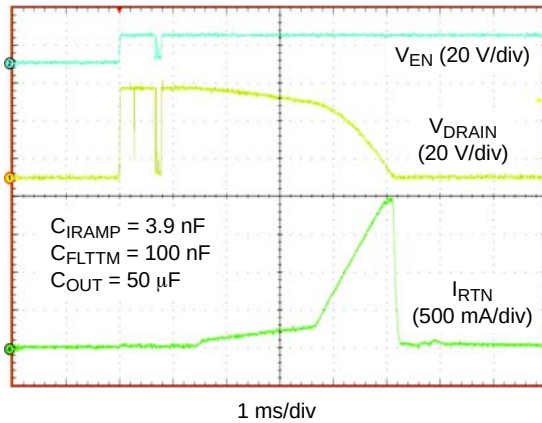
Figure 3. Live Insertion Event, V_{IN} = -48 V
