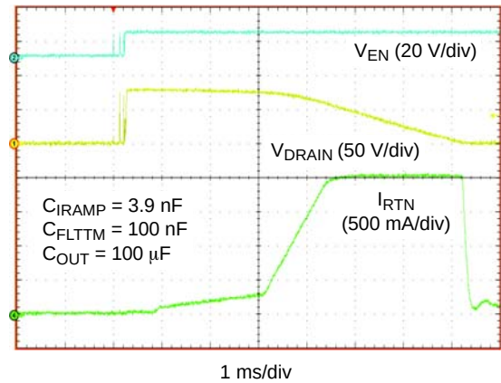
Figure 4. Live Insertion Event, V_{IN} = -80 V
