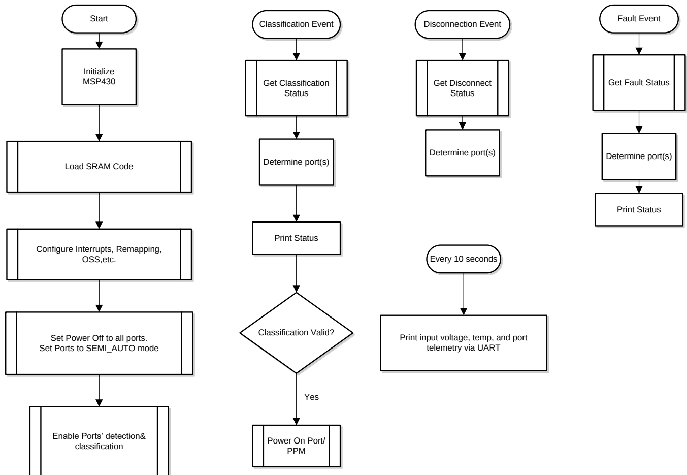
Figure 12. Semi Auto Mode System Software Structure
