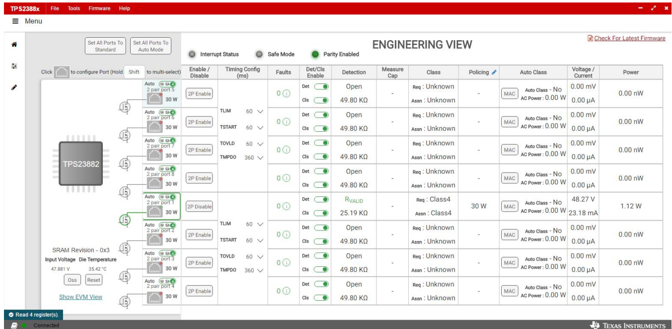
Figure 7. Device Configuration and Port Telemetry Page
