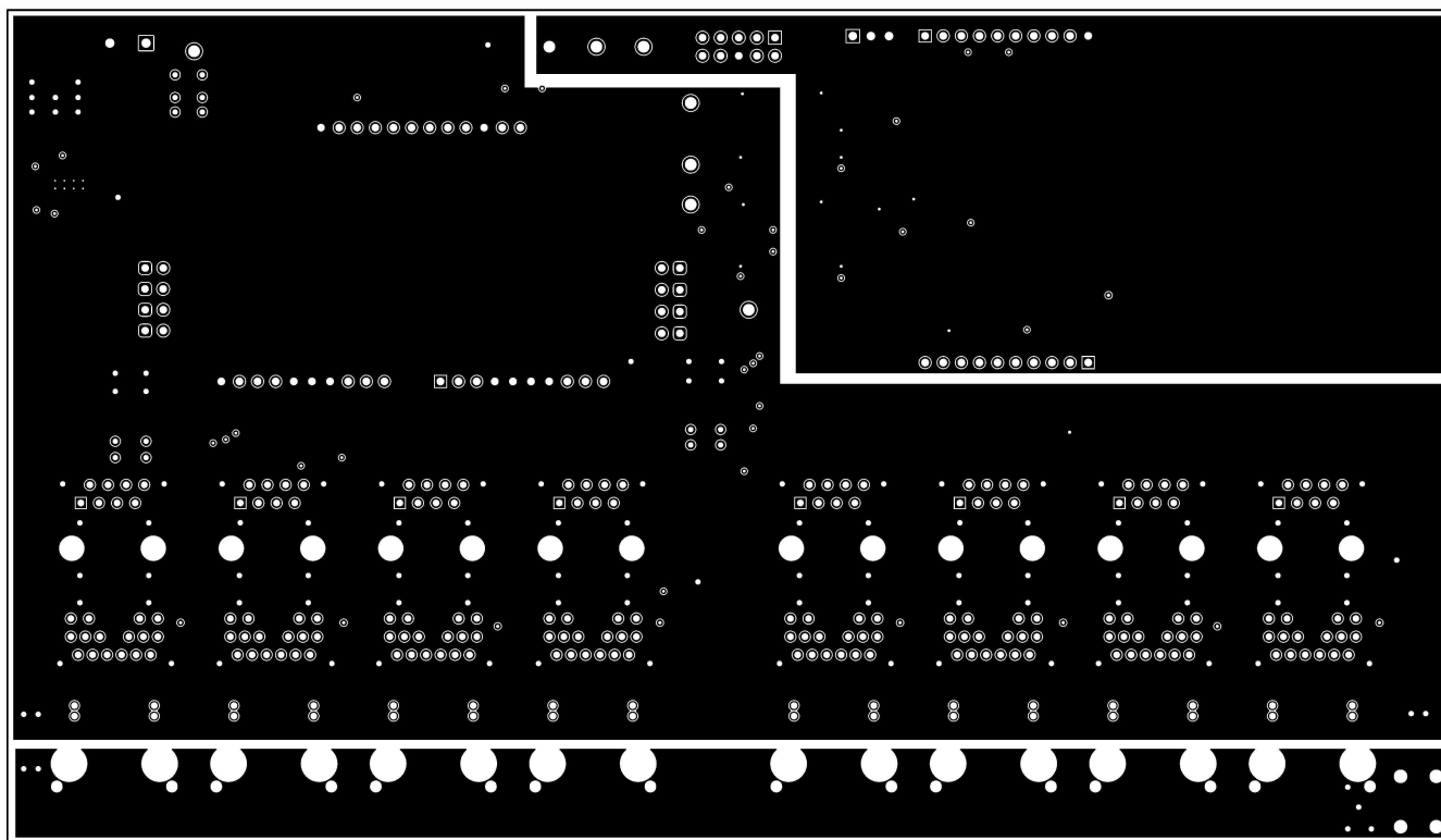
Figure 18. BOOST-PSEMTHR8-097 (Motherboard) Layer 2 Routing
