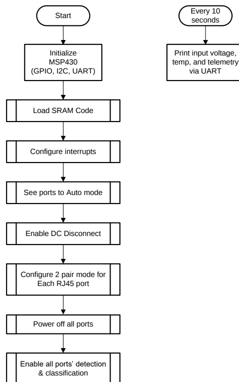
Figure 11. Auto Mode System Software Structure
