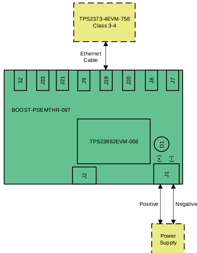
Figure 1. Basic Setup Using Autonomous Mode
