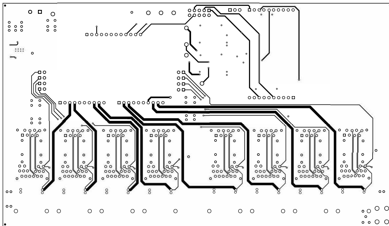
Figure 20. BOOST-PSEMTHR8-097 (Motherboard) Bottom Side Routing
