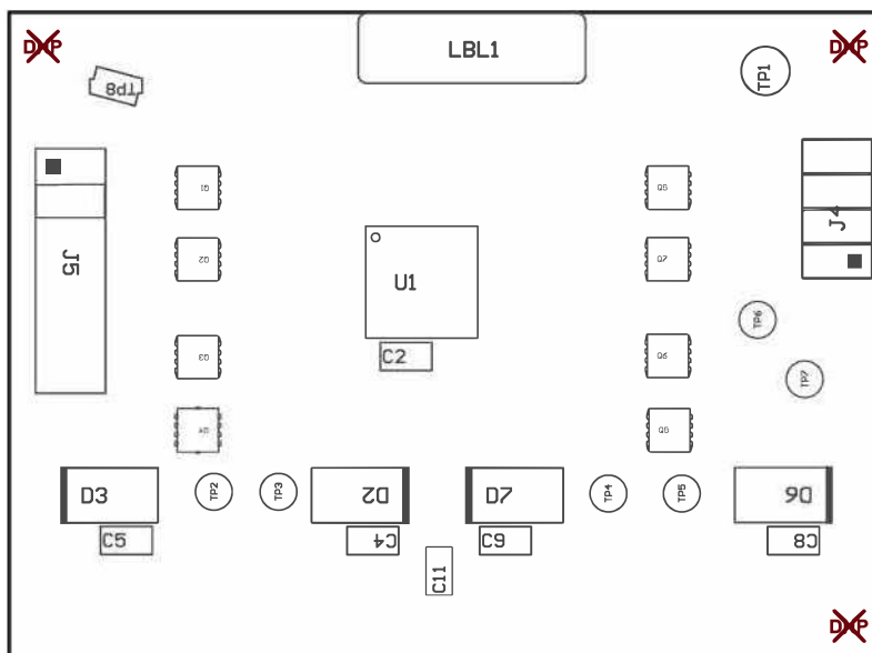
Figure 21. TPS23882EVM-008 (Daughterboard) Top Side Assembly
