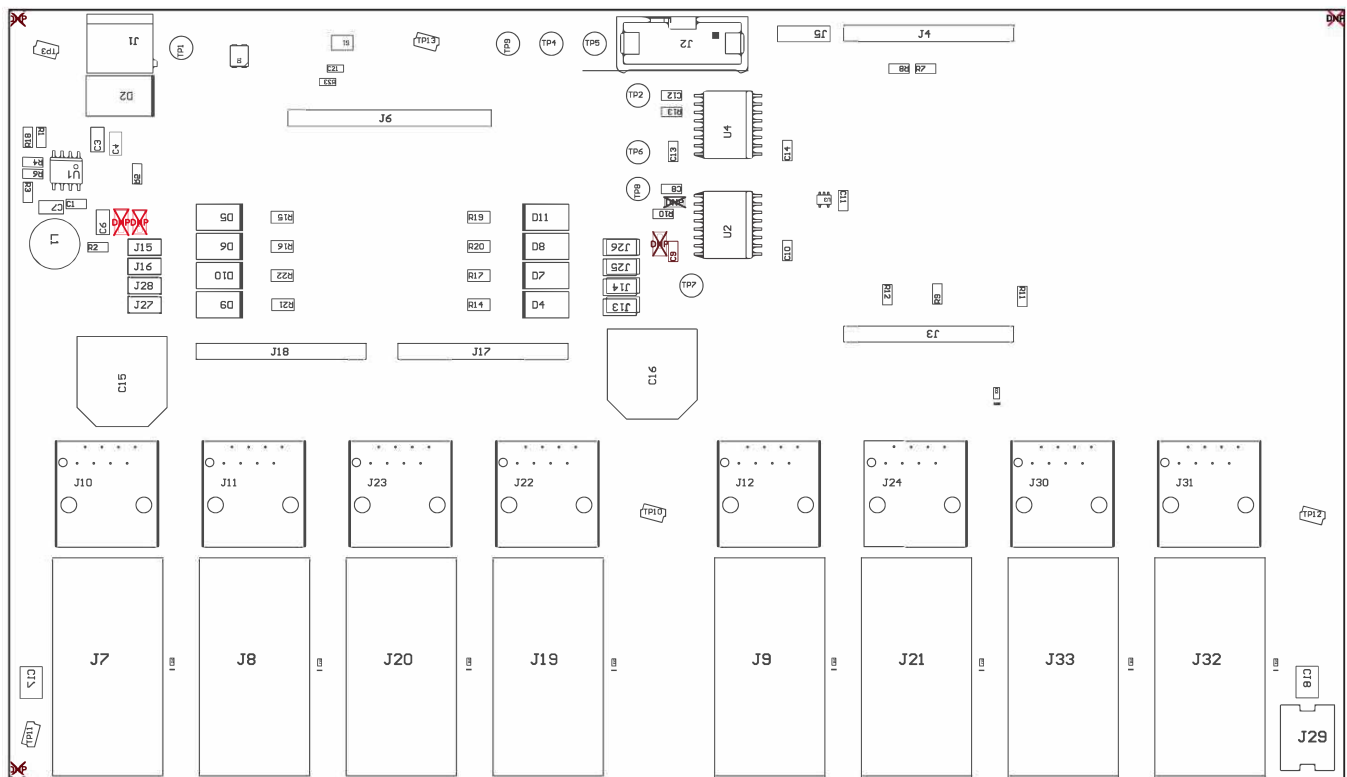
Figure 16. BOOST-PSEMT8-097 (Motherboard) Top Side Assembly
