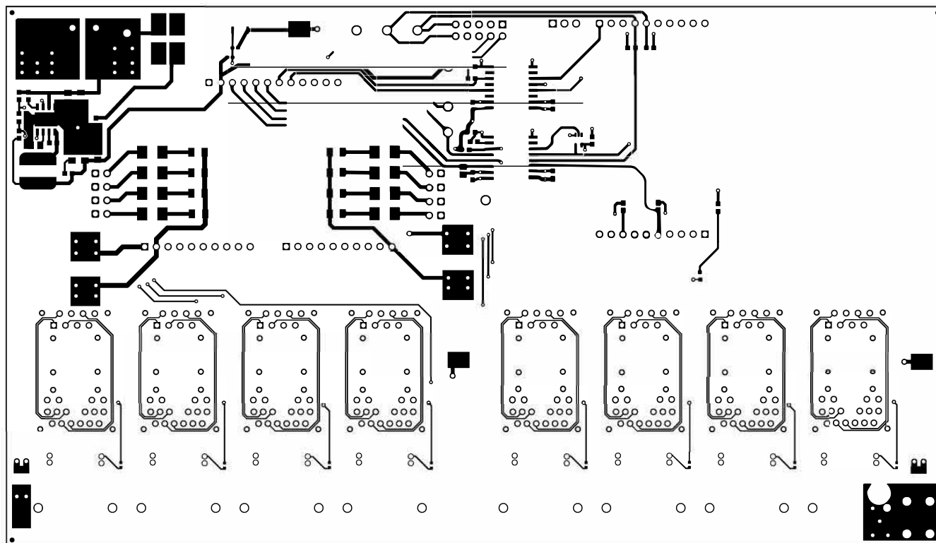
Figure 17. BOOST-PSEMTHR8-097 (Motherboard) Top Side Routing
