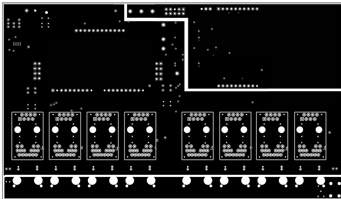
Figure 19. BOOST-PSEMTHR8-097 (Motherboard) Layer 3 Routing
