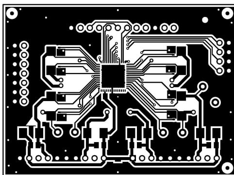
Figure 22. TPS23882EVM-008 (Daughterboard) Top Side Routing
