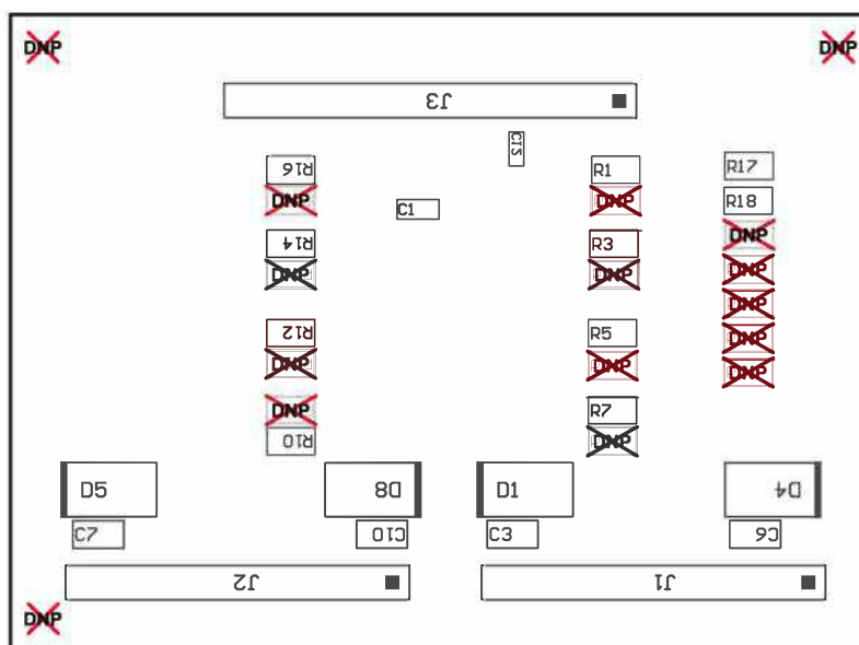
Figure 24. TPS23882EVM-008 (Daughterboard) Bottom Side Assembly
