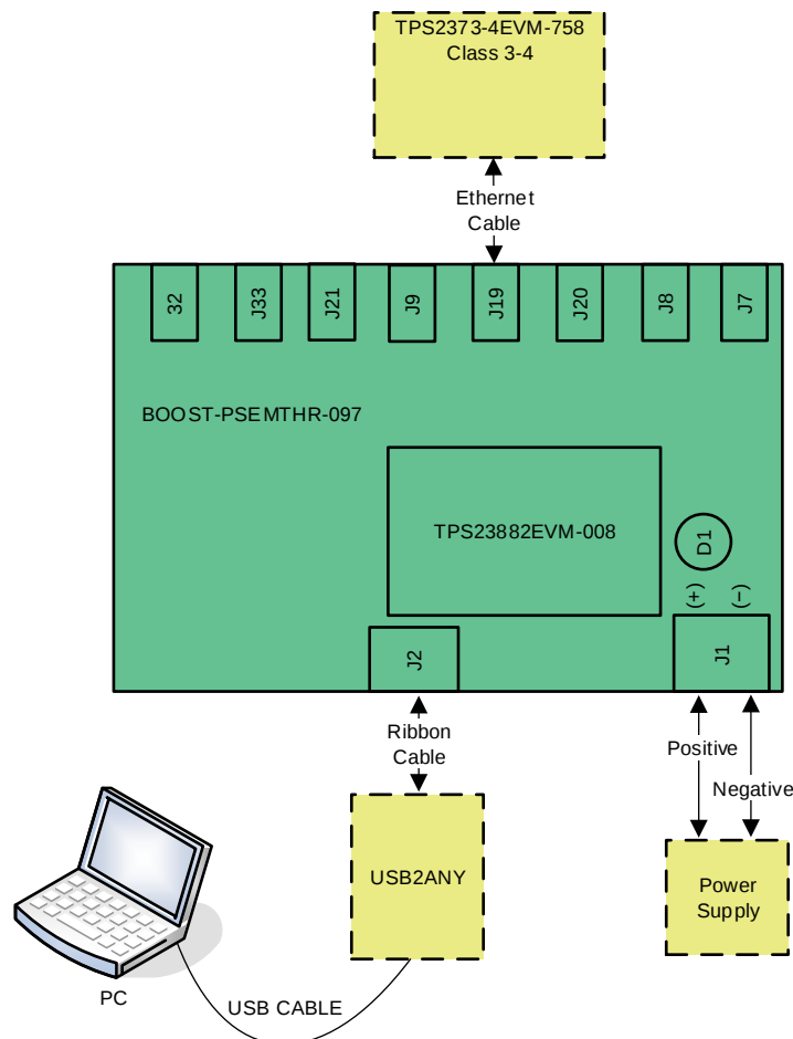
Figure 2. Basic Setup Using USB2ANY
