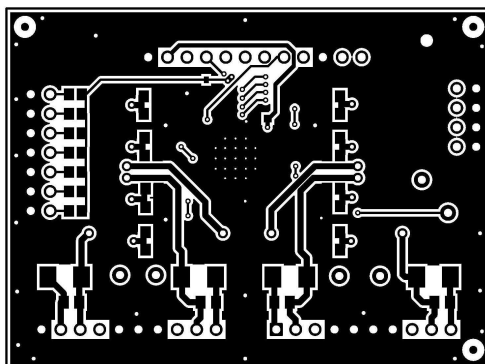
Figure 23. TPS23882EVM-008 (Daughterboard) Bottom Side Routing
