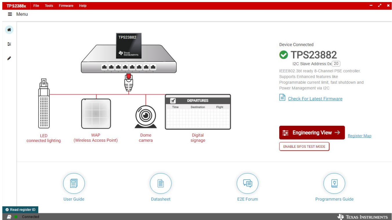
Figure 4. TPS23882 GUI Startup Window
