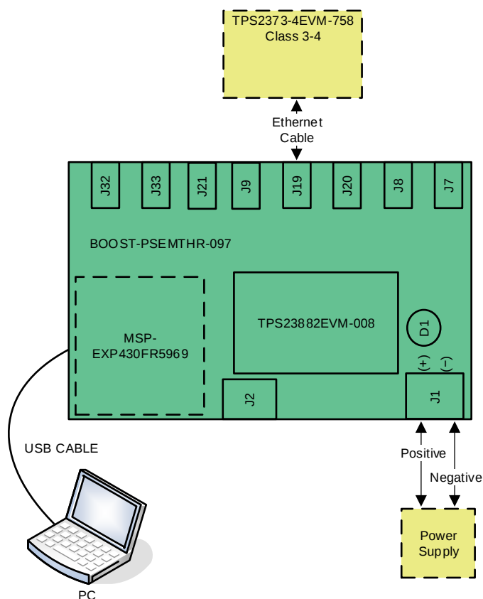
Figure 3. Advanced Setup Using LaunchPad™
