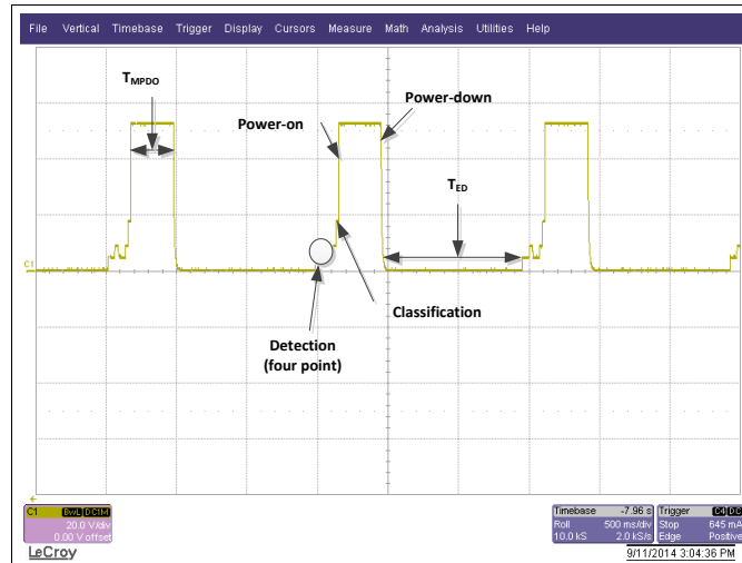
Figure 41. Good Detect, Class, Power-on, Followed by Under-current Disconnect
