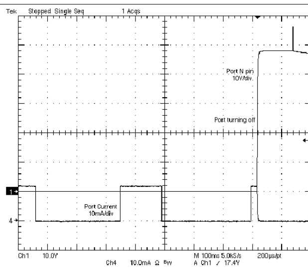
Figure 4. Port Under-current Response in DC Disconnect
