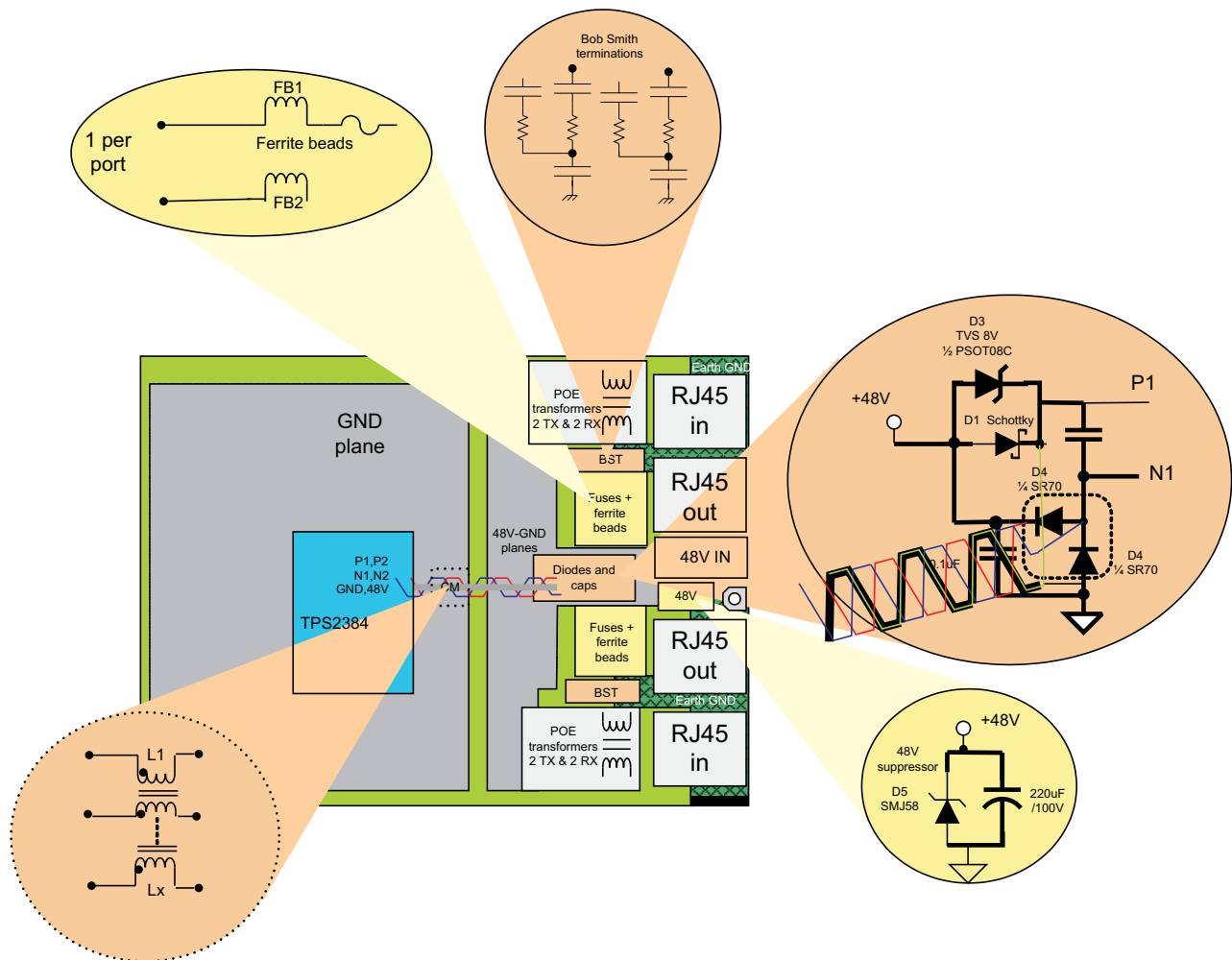
Figure 45. Layout
