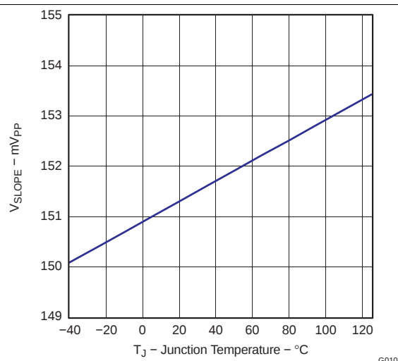
Figure 14. Current Slope Compensation Voltage vs Temperature
