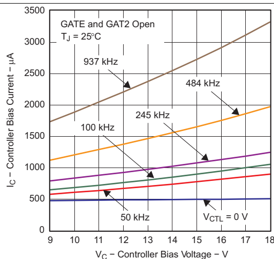
Figure 9. '754 Controller Bias Current vs Voltage
