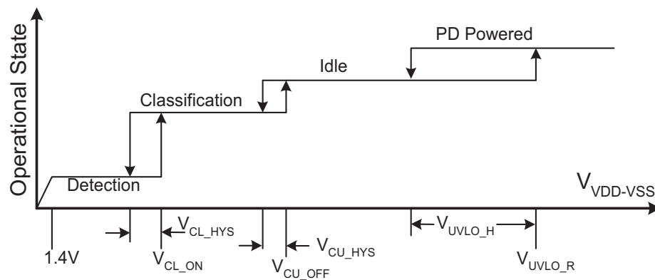
Figure 17. Threshold Voltages
