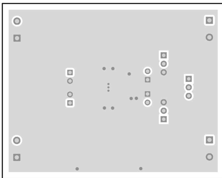
Figure 3. TPS22976EVM Bottom Layer
