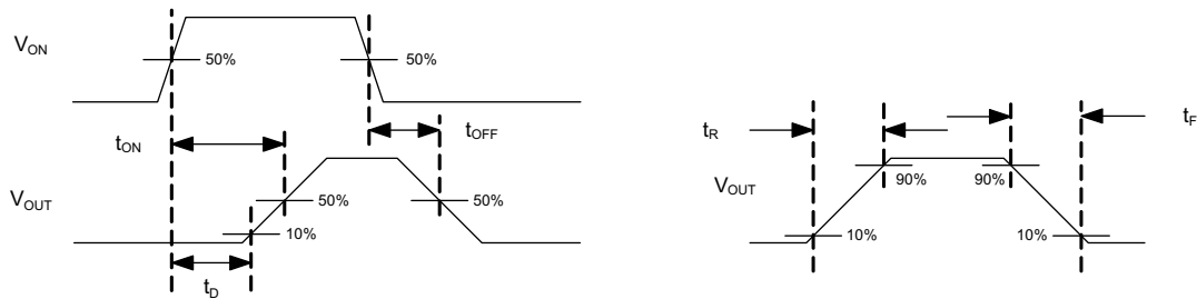
Timing Waveforms
