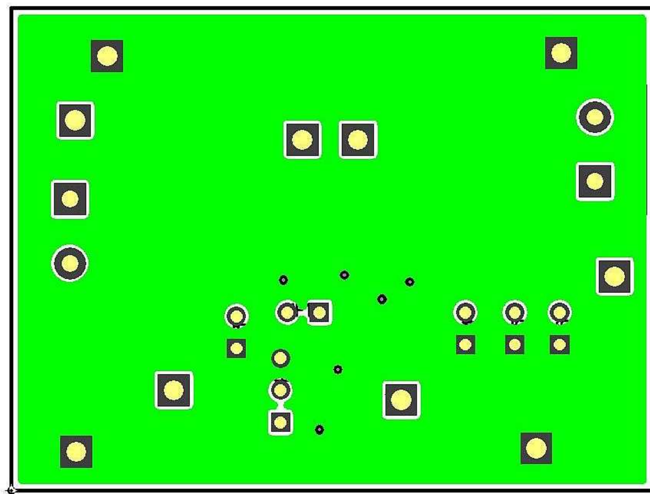
Figure 4. TPS22967EVM-023 Bottomside
