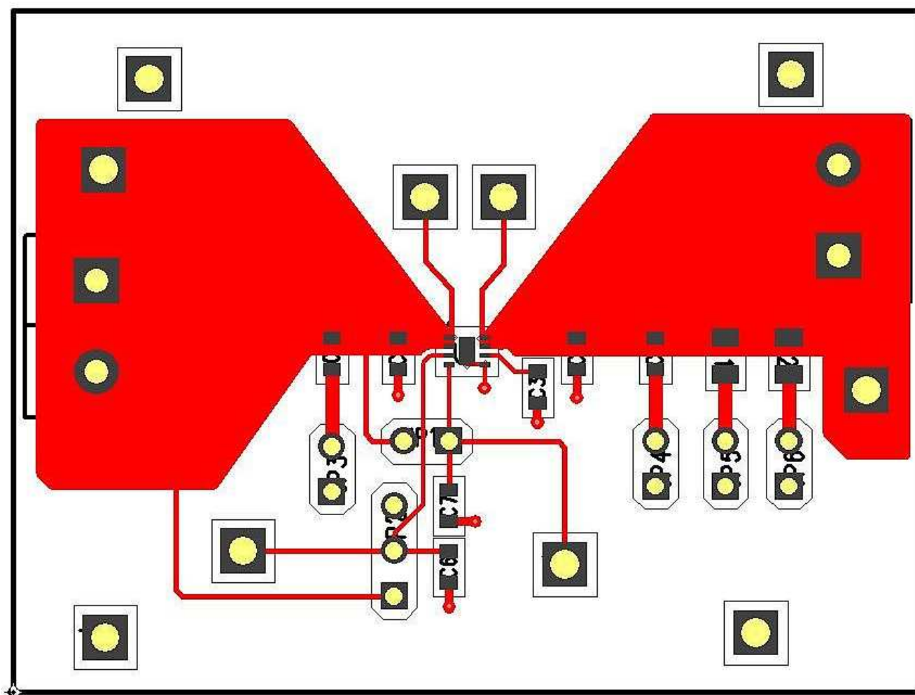
Figure 3. TPS22967EVM-023 Topside
